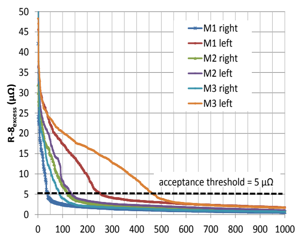
Figure 1. Excess joint resistance R_{8_{\text{excess}}} for the dipole (line M3) and quadrupole (line M1 and M2) busbars. Note that the two largest values (72 and 107 \mu\Omega ) are not shown [2].
