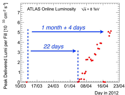
Figure 2: Luminosity versus time as recorded in ATLAS in the first weeks of the 2012 run. Courtesy of the ATLAS collaboration.
