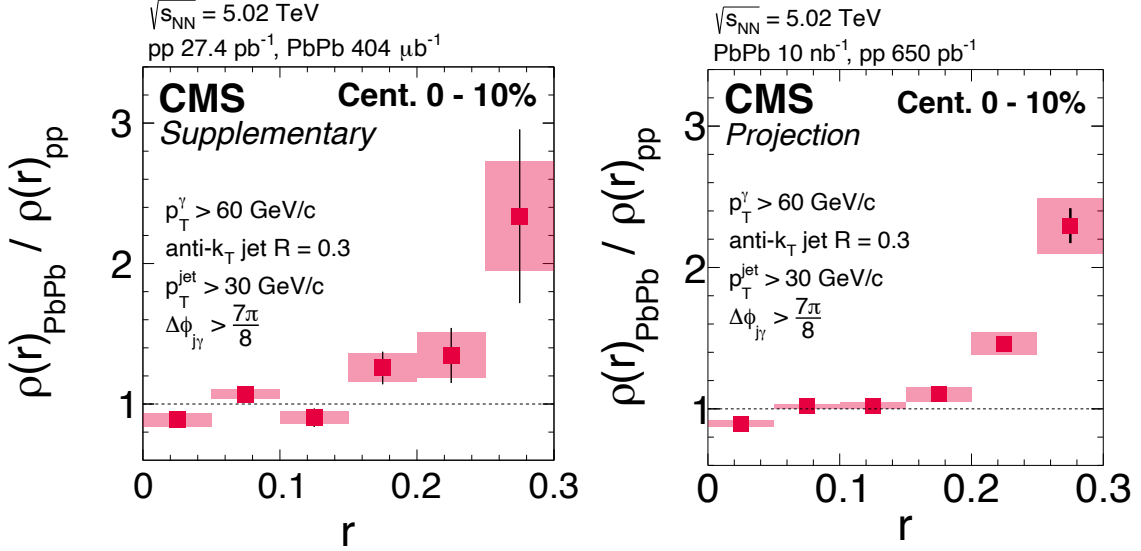
Fig. 34: (Left Panel:) The ratio of measured photon-tagged jet shape in Pb–Pb and pp collisions with the 2015 Pb–Pb data [395]. (Right Panel:) The expected performance of the jet shape ratio in the HL-LHC data, using a third-order polynomial for smoothing the data. [REF to be added when note is public]
