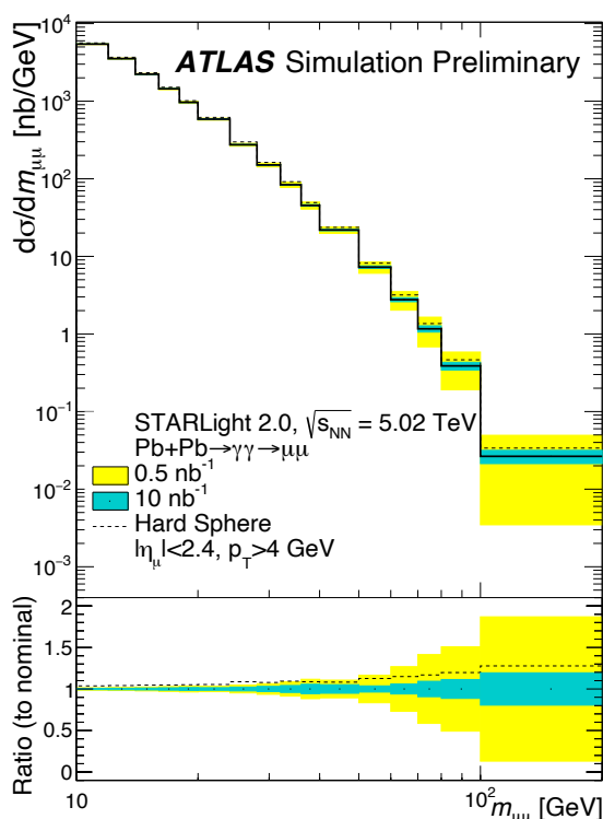
Fig. 98: (Upper) Differential cross section for exclusive production of the di-muon pairs as a function of the di-muon mass for 10 < m_{\mu\mu} < 200 \text{ GeV} extracted from STARLight. Two scenarios are considered for the nuclear geometry: a realistic skin depth of the nucleus (solid line) or a hard sphere (dashed line). (Bottom) Ratio to nominal as a function of the di-muon mass, where "nominal" stands for the realistic skin depth of the nucleus. Shaded bands represent expected statistical uncertainties associated with a number of signal events in each bin for integrated luminosity of 0.5 \text{ nb}^{-1} (yellow), and 10 \text{ nb}^{-1} (cyan).
