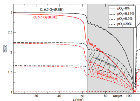
Fig. 27: Comparison of the computed oxygen-enhancement ratio (OER) along a spread-out Bragg peak (SOBP) for carbon (black curves) and oxygen (red curves) at different levels of partial O_2 pressure. The hatched areas represent the clinically interesting regions for hypoxia ( 0.15\% < pO_2 < 0.5\% ). The indicated doses are prescribed RBE-weighted doses in the target to achieve isosurvival.
