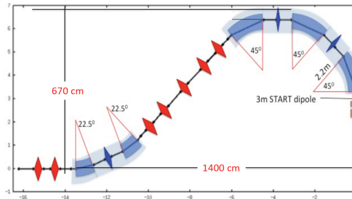
Fig. 68: Sigrum gantry, conservative version, with 3-T SC magnets. This requires two 22.5^\circ bending magnets (contained in the first cryostat) and three 45^\circ bending magnets (contained in the second cryostat).
