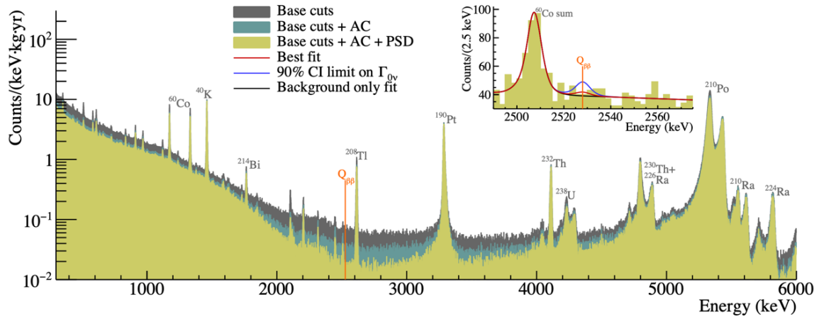
Fig. 32-13: The CUORE physics spectrum 1123 , with zoom on the region of interest.
