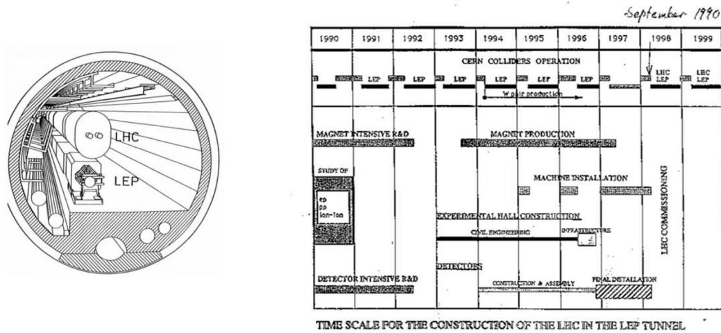
Fig. 22-5: The 1990 planning of LHC coexisting with LEP 652 . The left figure is from Ref. 653 .
