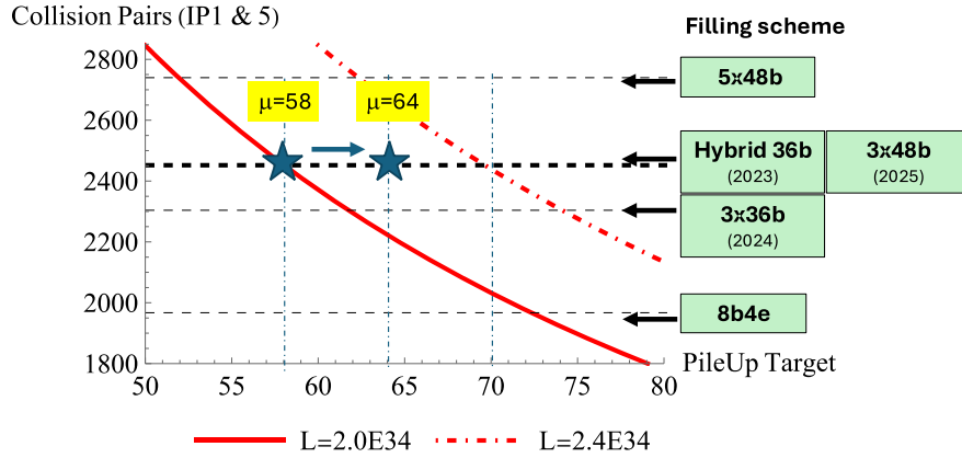
Fig. 21-6: The number of colliding bunches in the interaction points IP1 (ATLAS) and IP5 (CMS) as a function of the pile-up ( \mu ) during Run 3 of the LHC. The red lines indicate lines of fixed instantaneous luminosity (units of \text{cm}^{-2}\text{s}^{-1} ). There are 3564 possible bunch positions every 25ns in the circumference of the LHC ring: “b” indicates a position with beam and “e” indicates an empty position. On the right side, the various LHC filling schemes considered in Run 3 are indicated, pointing to the number of colliding bunches they contain. Each year, one used the filling scheme that provided the maximal number of bunches compatible with the beam screen heating due to the electron-cloud effect 643 .
