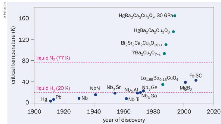
Fig. 23-7: Discovery of HT superconductors versus year 668 .
