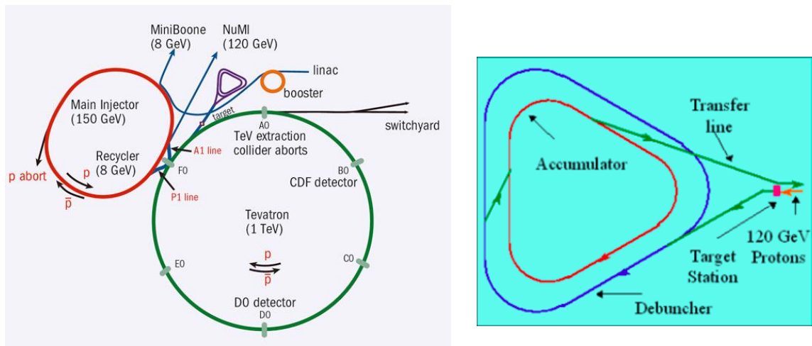
Fig. 10-13: Fermilab accelerator chain (left) and the Tevatron antiproton source (right).
