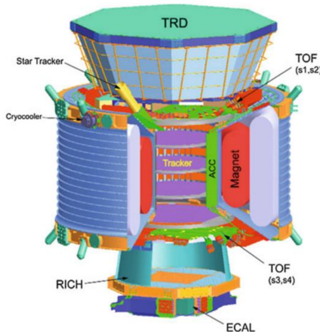
Fig. 35-6: AMS detector on the ISS showing the main sub-detector elements and their functions.
