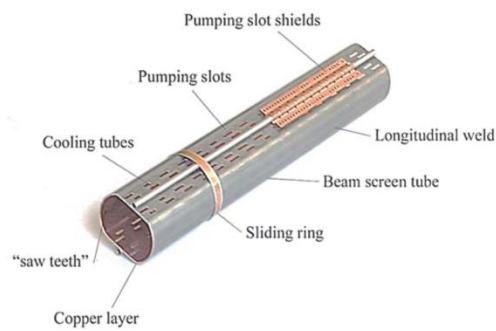
Fig. 23-5: Beam screen and vacuum tube coating 666 .
