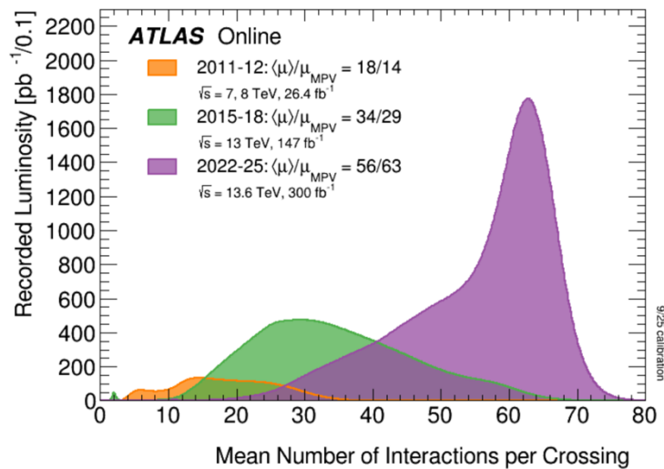
Fig. 21-7: Beam conditions for ATLAS: luminosity-weighted distribution of the mean number of interactions per crossing as measured by ATLAS. the mean \mu value, and the most probable (MPV) \mu value are given for data taking periods from 2011 till 2025.
