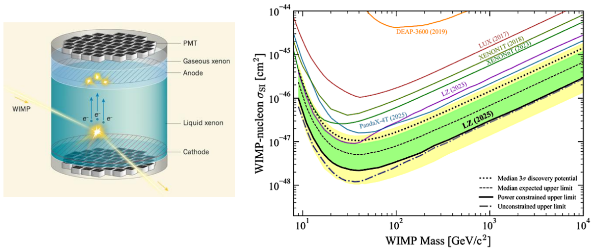
Fig. 31-21: Dual-phase Xenon detection technology (left) and present upper limits (90% CL) on the spin-independent WIMP-nucleon cross-section as a function of WIMP mass from different experiments (right) 1026 .
