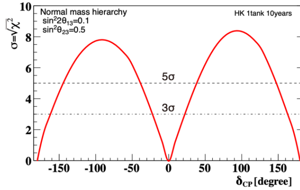
Fig. 19-14: Expected significance of exclusion of \sin \delta_{CP} = 0 528 .
