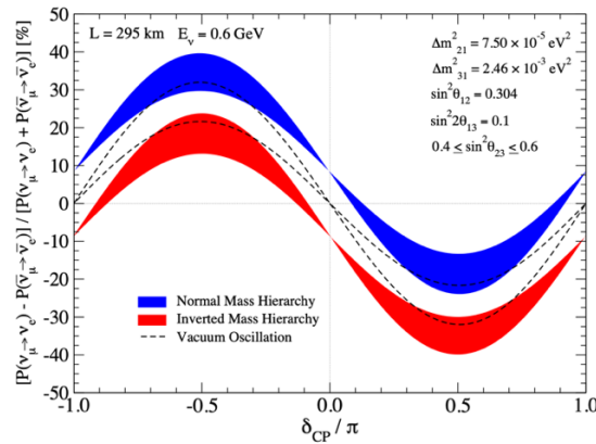
Fig. 19-13: Effect on the neutrino/antineutrino rate difference 527 .
