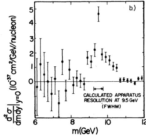
Fig. 13-7: Beauty discovery: Measured dimuon production cross-sections as a function of the invariant mass of the muon pair 336 .
