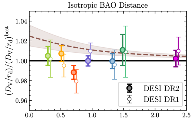
Fig. 30-16: DESI results: abscissa is the redshift; r_d is the scale of the pre-recombination sound horizon; D_V is the isotropic BAO distance 947 .
