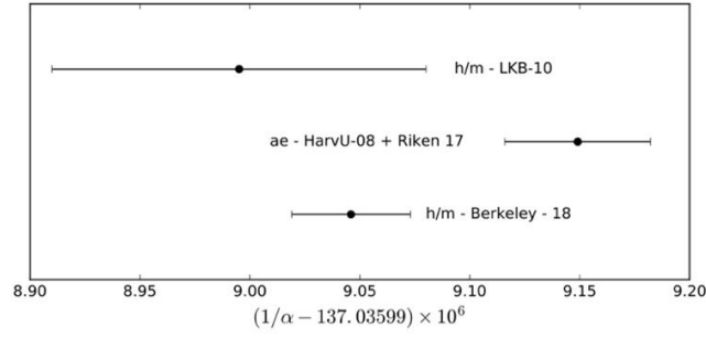
Fig. 26-17: Three best determinations of \alpha from h/m and from a_e 846 .
