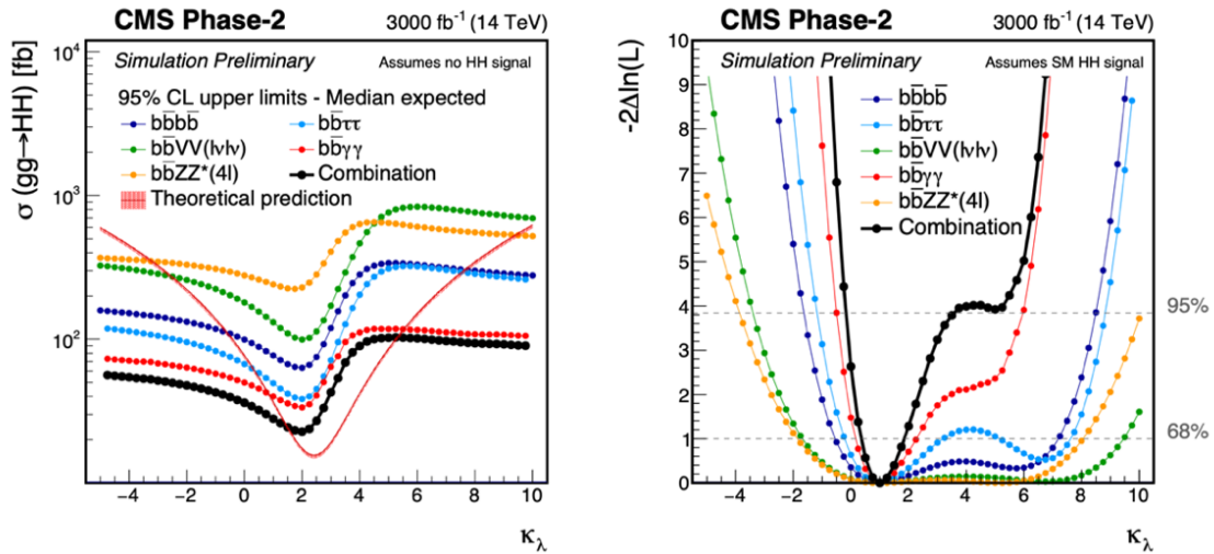
Fig. 24-13: The plots suggest what the HL-LHC will bring for the self-interaction coupling modifier \kappa_\lambda 713 . Left: upper limit at the 95% CL on the HH production cross section as a function of \kappa_\lambda . The red band indicated the theoretical production cross section. Right: expected likelihood scan as a function of \kappa_\lambda . For explanations of the patterns of the curves see 714 .
