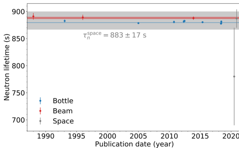
Fig. 32-34: The neutron lifetime measurements 1184 .
