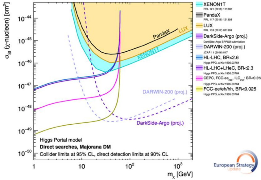
Fig. 31-24: Future colliders limits (direct searches for Higgs invisible decays) with constraints from current and future direct detection experiments on the spin-independent WIMP– nucleon scattering cross-section for a simplified model with the Higgs decaying to invisible (DM) Majorana particles 1029 .
