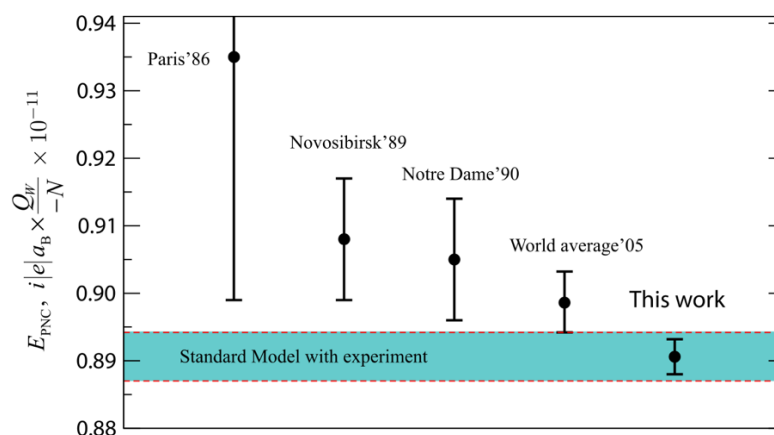
Fig. 25-3: Progress in evaluating the parity non-conserving (PNC) amplitude.
