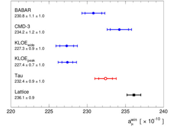
Fig. 26-8: Some tension between KLOE and other results 833 ?
