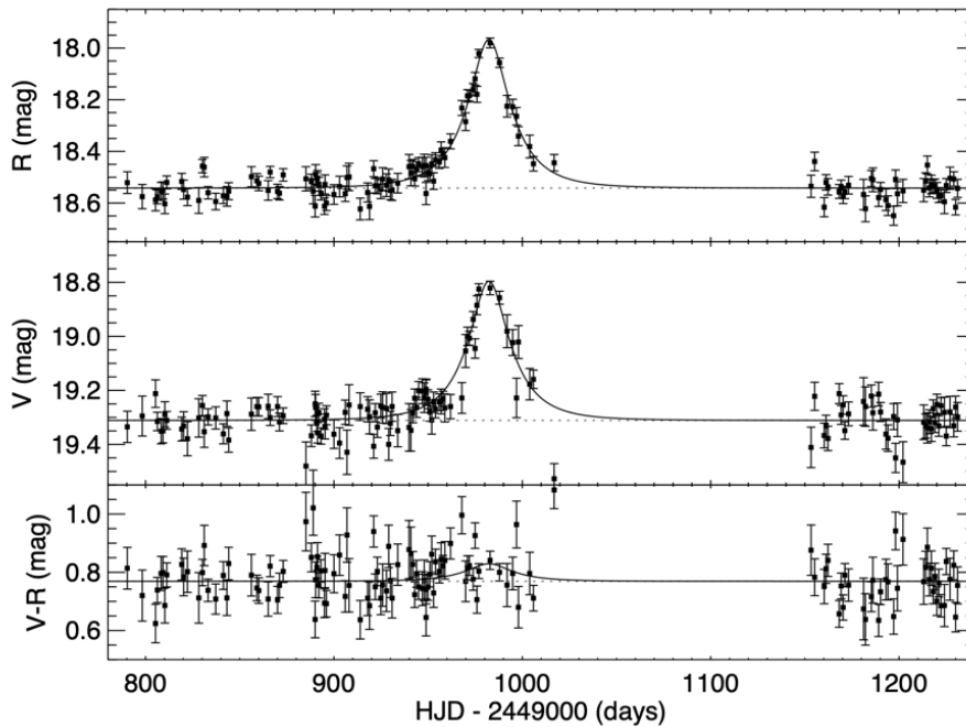
Fig. 31-47: A microlensing event. Light curve of the MACHO-95-BLG-37 event 1082 .
