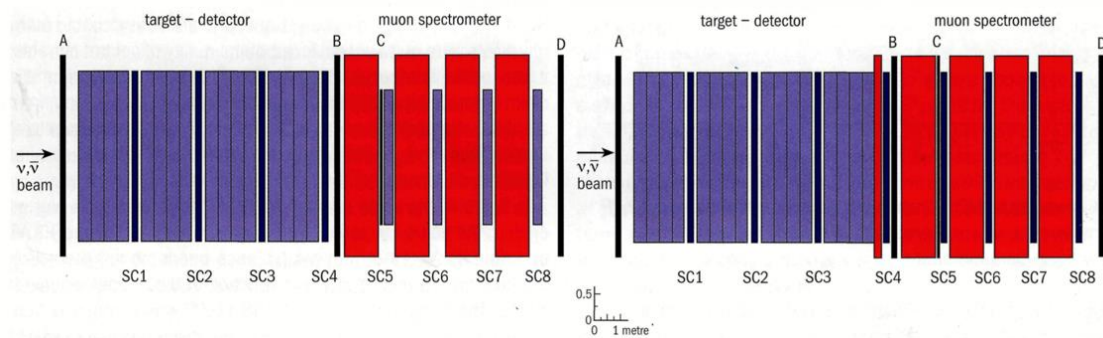
Fig. 9-9: HPWF experiment before (left) and after (right) modifications 216 .
