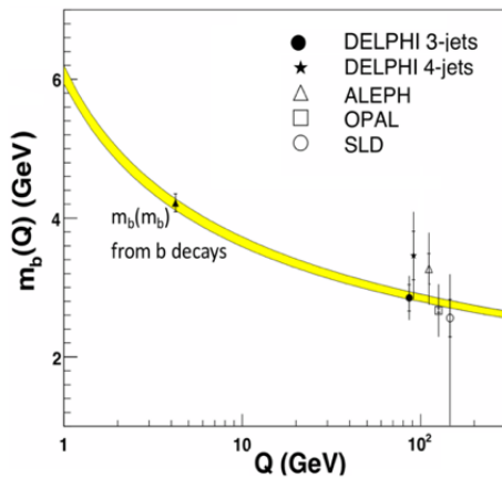
Fig. 16-8: The variation of m_b with energy 429 .
