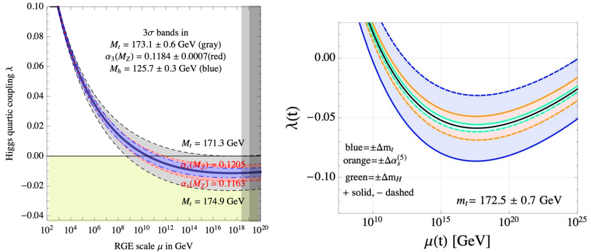
Fig. 24-17: Evolution of the quartic coupling with RGE scale: left from Ref. 721 , right from Ref. 722 .
