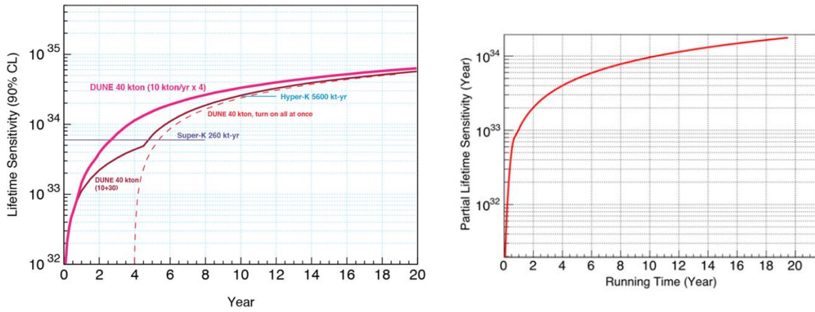
Fig. 32-32: Sensitivities of DUNE and HyperK 1167 (left) and sensitivity of JUNO 1168 (right).
