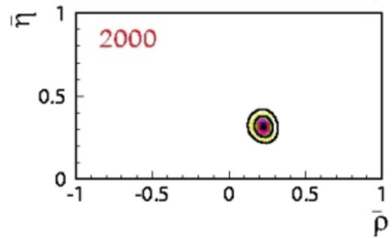
Fig. 16-9: Evidence of CP violation in B sector 430 .
