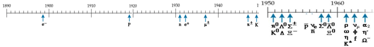
Fig. 4-1: The 1950s avalanche 28 .
