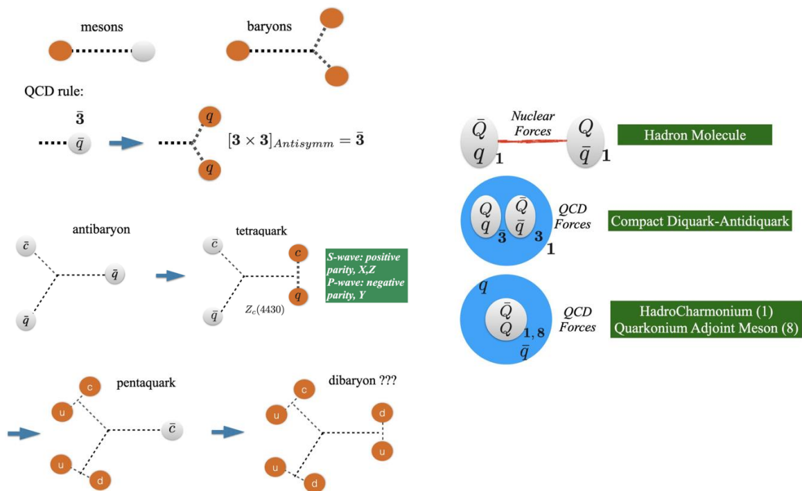
Fig. 28-2: How to make coloured singlets: colour strings in ordinary particles, colour strings in multiquark states (left) and scheme of hadronic molecules, compact tetraquarks, HadroCharmonium (right).
