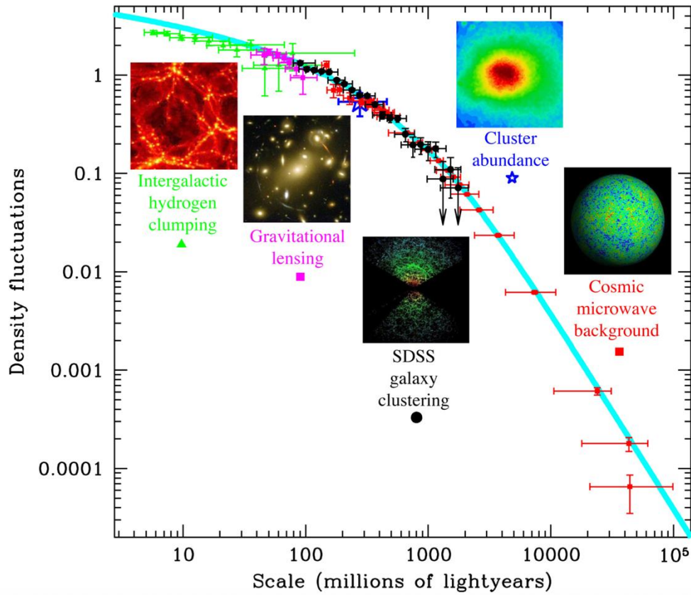
Fig. 31-5: Another view of the power spectrum of density fluctuations in the Universe 995 . The y-axis labelled “Density fluctuations”, shows the power spectrum in dimensionless form, as the variance per logarithmic interval in k , \Delta^2(k) \propto k^3 P(k) . The x-axis is the comoving scale (1 Mpc \sim 3.3 Mly). Different tracers of the density are used on different scales. The turquoise curve shows a fit to the data with the parameters of the standard \Lambda CDM cosmological model (Figure credit: M. Tegmark, MIT).
