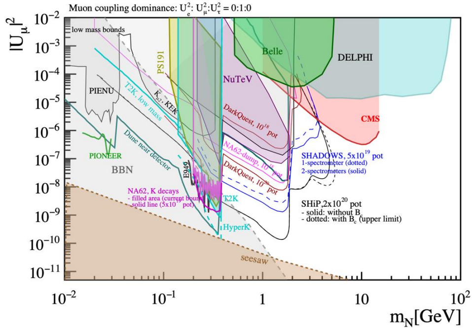
Fig. 19-27: HNL with couplings to the 2 nd generation. Filled areas are existing bounds. Coloured curves are projections 562 .
