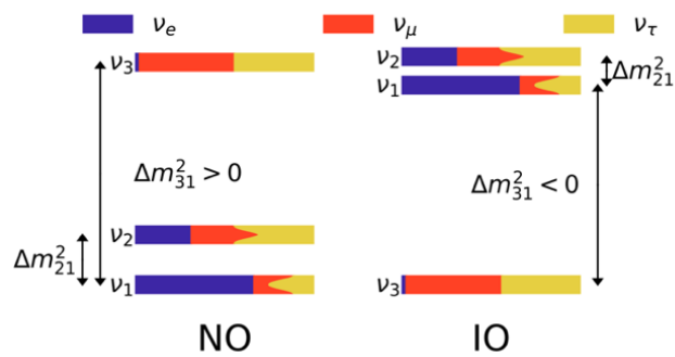
Fig. 19-7: Possible ordering of the neutrino mass spectrum 514 .
