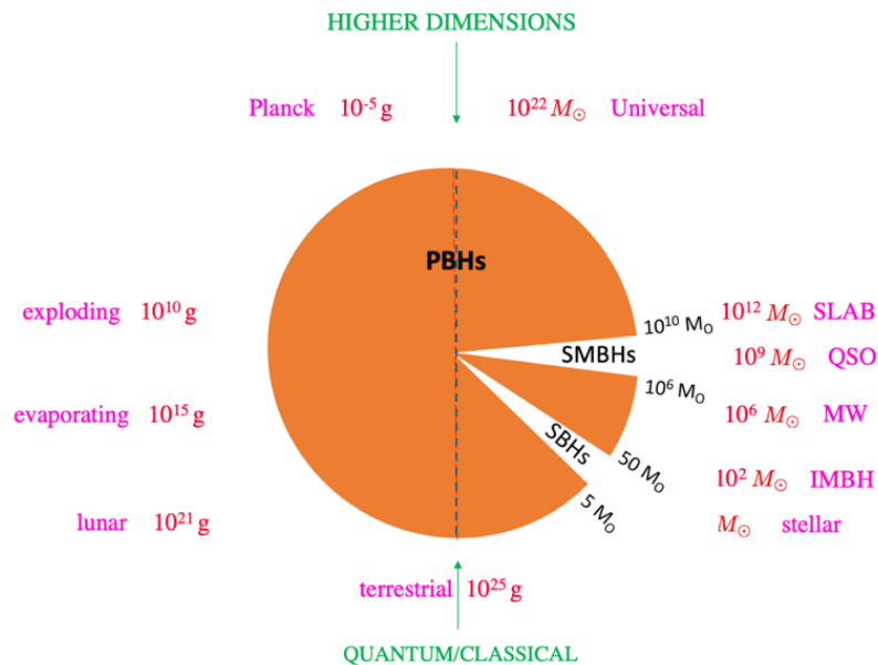
Fig. 31-51: This diagram indicates the mass of various types of black holes. Quantum emission is suppressed by accretion of the CMB to the right of the bottom point.
