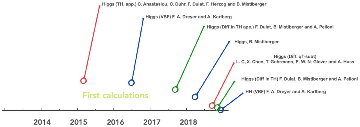
Fig. 5-23: Steps of the N 3 LO revolution for Drell–Yan like processes 78 .
