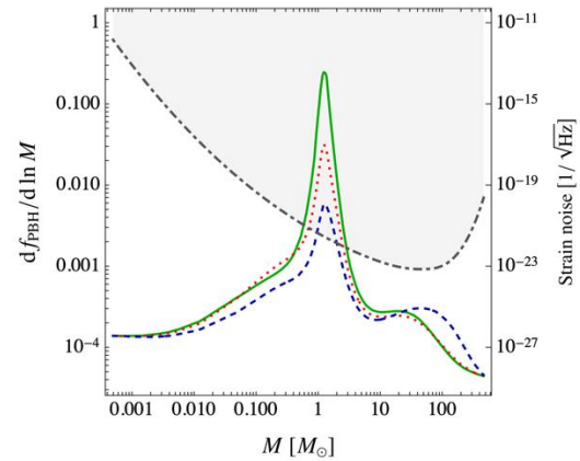
Fig. 31-55: Spectral density of the PBH dark matter fraction as a function of PBH mass. The green solid line indicates the standard scenario. Also shown is the LIGO sensitivity curve (grey dot-dashed line) for equal-mass mergers and using the maximal GW frequency f_{\text{max}} \approx 4400 M_{\odot}/M for the conversion from frequency to mass 1098 .
