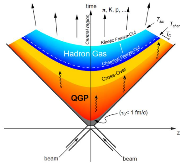
Fig. 20-1: The successive stages 599 .
