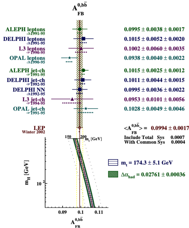
Fig. 18-3: LEP results on A_{FB}^{0,b\bar{b}} , see Ref. 459 .
