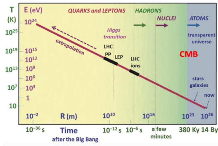
Fig. 30-2: Left: the Universe timeline; right: above the Friedmann equation with Euclidean 3-space; below the second Friedmann equation ( p is pressure).
