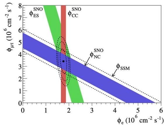
Fig. 19-5: Results from SNO.
