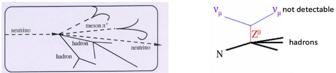
Fig. 9-6: Events without a charged lepton and their interpretation.
