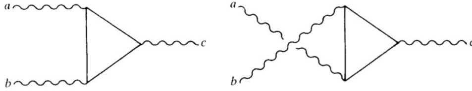
Fig. 7-3: Potentially anomalous couplings of currents a, b and c by a fermion triangle loop 171 .
