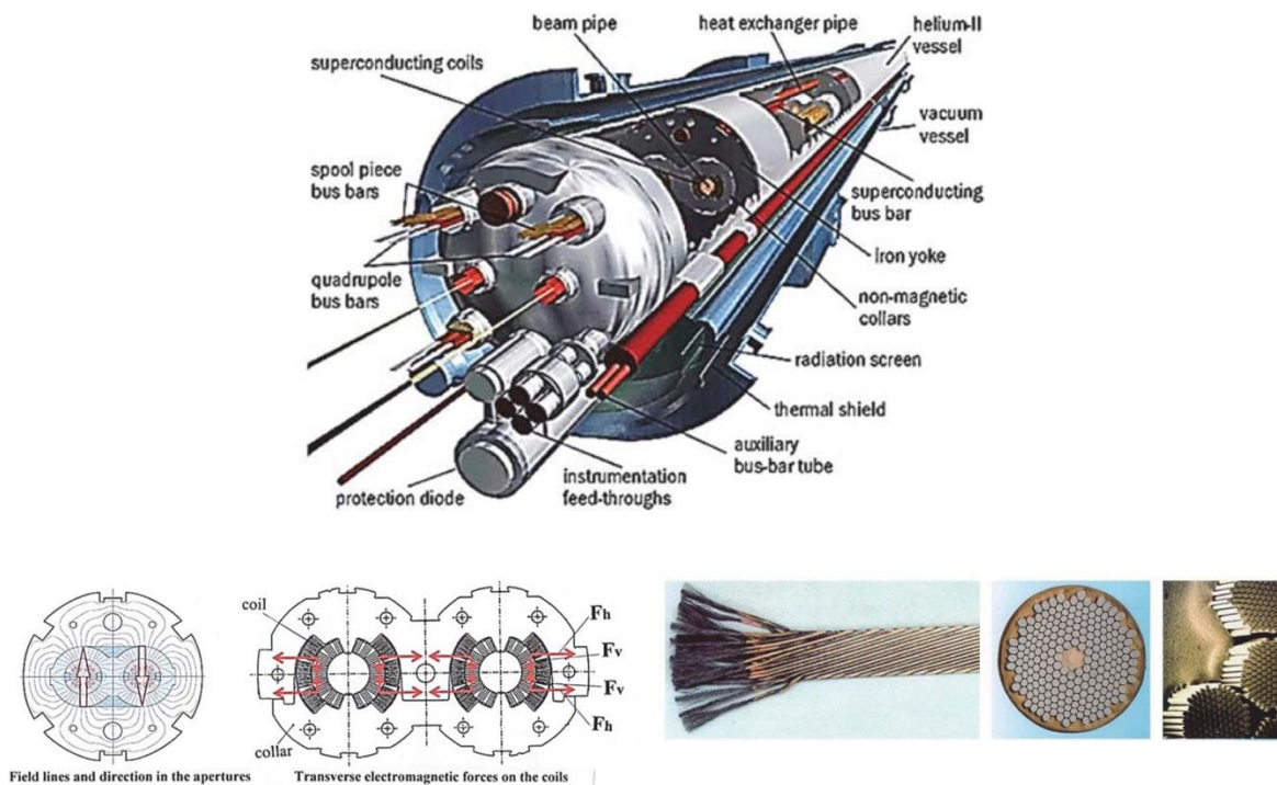
Fig. 23-4: The LHC magnets 665 . Top: cut-away view of the 15 m long superconducting dipole. Bottom left: field and forces in the twin aperture magnet. Bottom right: a flat LHC cable, a strand and groups of Nb-Ti filaments in a strand.
