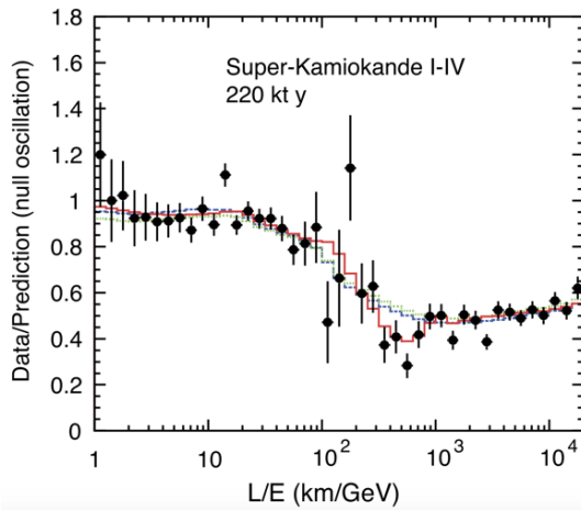
Fig. 19-4: The ratio of data to MC events (in the absence of neutrino oscillation) as a function of the reconstructed L/E .
