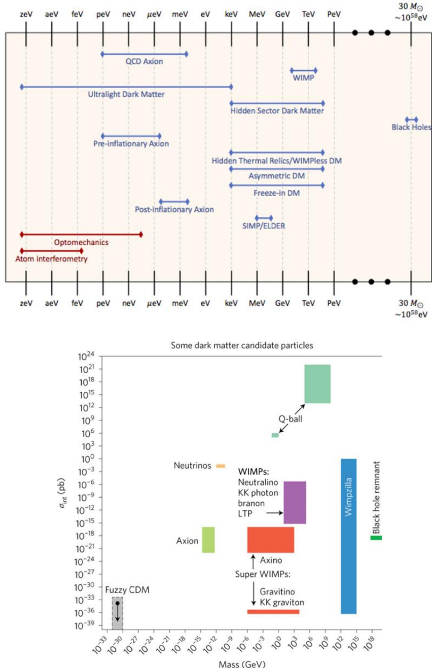
Fig. 31-10: The variety of hypotheses on the nature of DM. Top: Figure taken from Ref. 1012 . Summary of some among the dark matter candidates and their mass compared to the range of parameters covered by atom interferometry and optomechanical set-ups, proposed to test light DM candidates. Bottom: Figure taken from Ref. 1013 .
