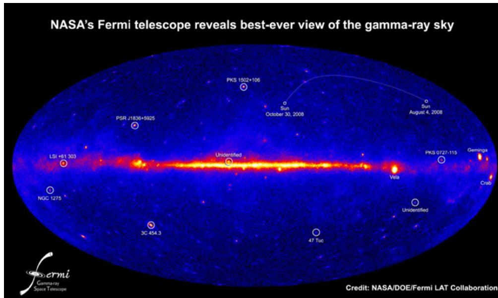
Fig. 35-10: The image shows how the sky appears at energies more than 150 million times greater than that of visible light 1238 .
