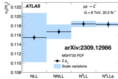
Fig. 5-14: Improvements on \alpha_s(M_Z) 66 .
