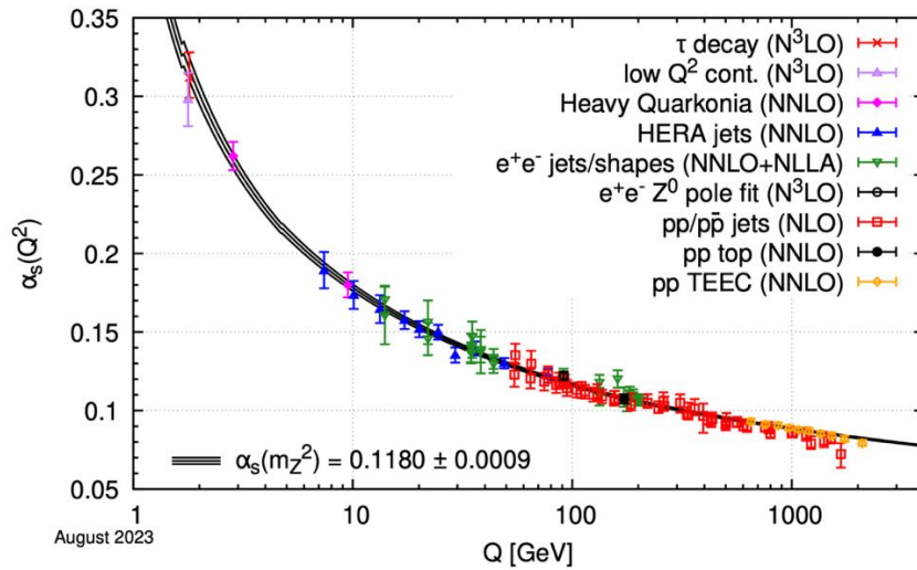
Fig. 5-11: The key facts of QCD: Summary of determinations of \alpha_s as a function of the energy scale Q compared to the predicted running of the coupling \alpha_s 57 .
