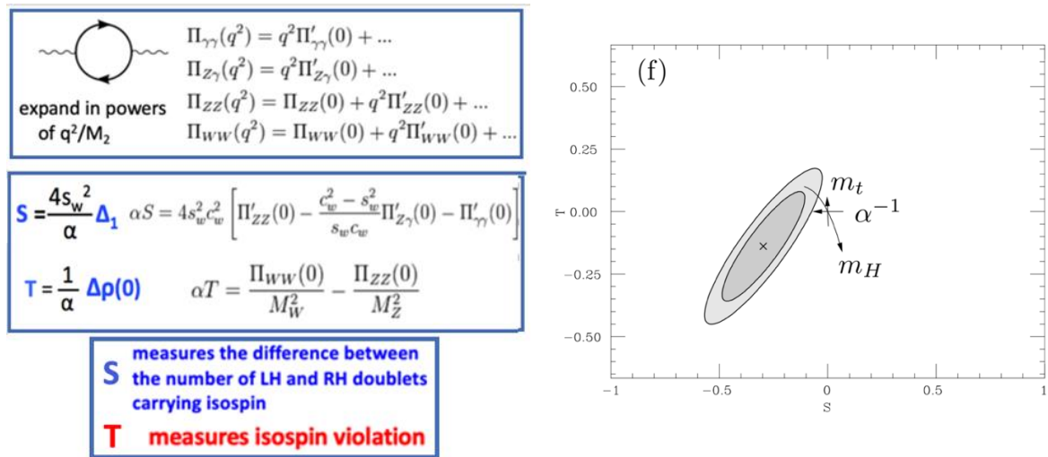
Fig. 18-11: Left: properties of the global variables S, T: The \Pi are vacuum polarization functions. Figure built from Ref. 470 . Right: LEP results seen in the S-T plot 471 .
