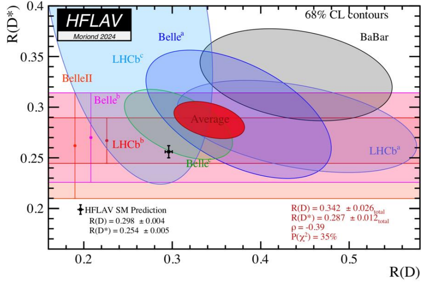
Fig. 14-5: R(D^*) measurements 344 .
