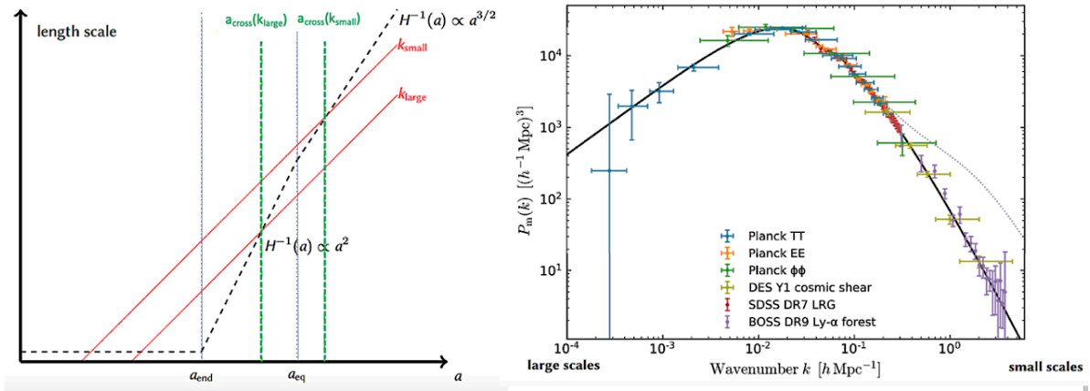
Fig. 31-4: Left: dependence of scales k^{-1} on their time a_{\text{cross}} of crossing the Hubble radius H^{-1}(a) . Right: the matter power spectrum 994 .
