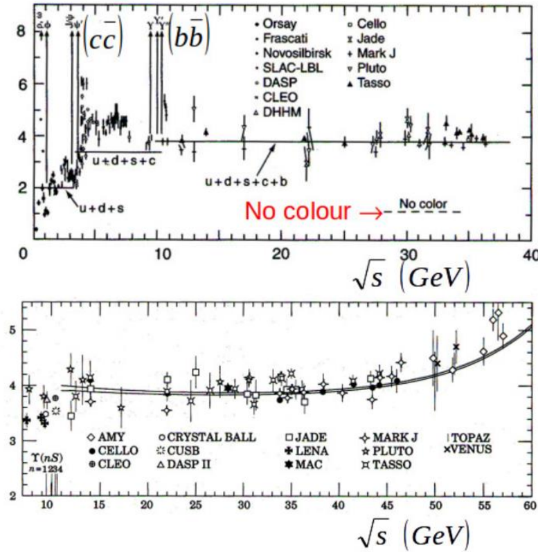
Fig. 5-12: Two views of the R ratio R = \frac{\sigma(e^+e^- \rightarrow \text{hadrons})}{\sigma(e^+e^- \rightarrow \mu^+\mu^-)} shown in the y-axis (from T. Potter 59 ).
