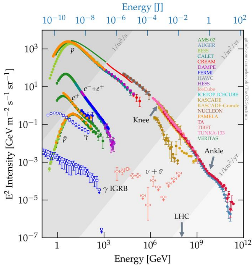
Fig. 19-36: The overall cosmic ray scenery 594 .
