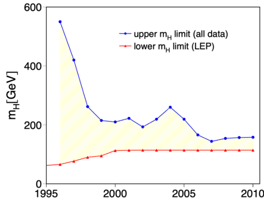
Fig. 18-1: Indication of Higgs mass from LEP 456 .
