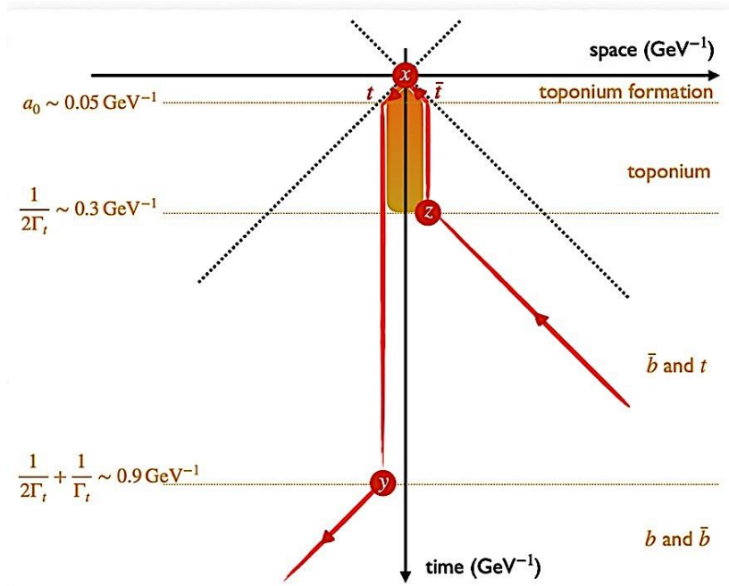
Fig. 24-48: A position space picture of toponium 802 .
