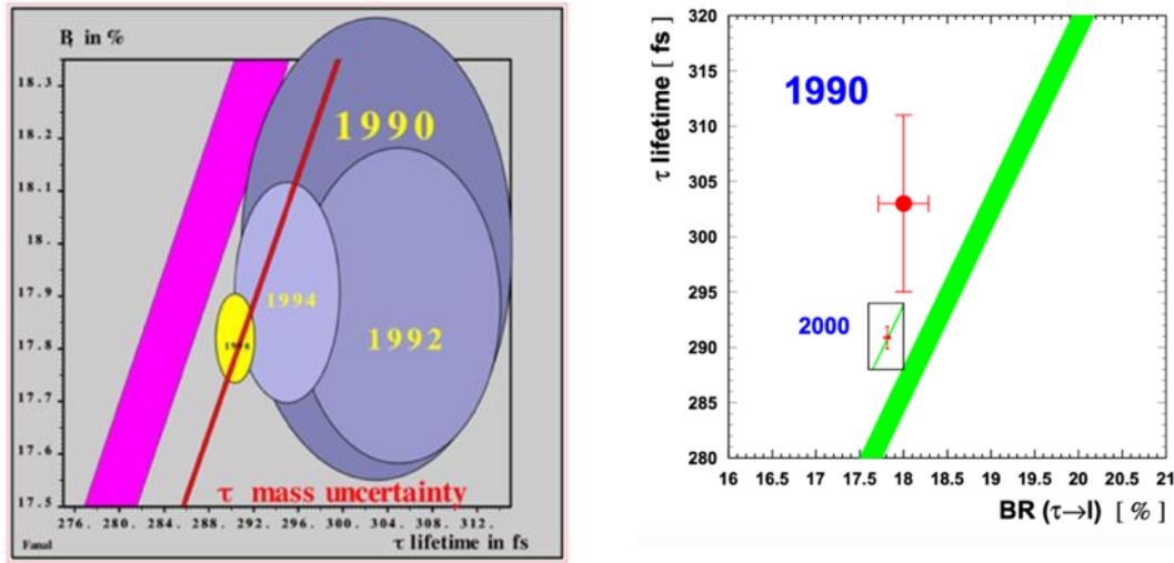
Fig. 16-10: The \tau is a normal lepton. Left: courtesy H. Videau. Right: from Ref. 431 .
