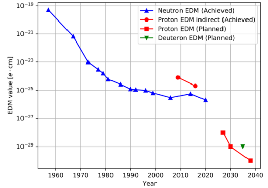
Fig. 32-17: Limits of n, p and deuteron EDM versus time 1131 .
