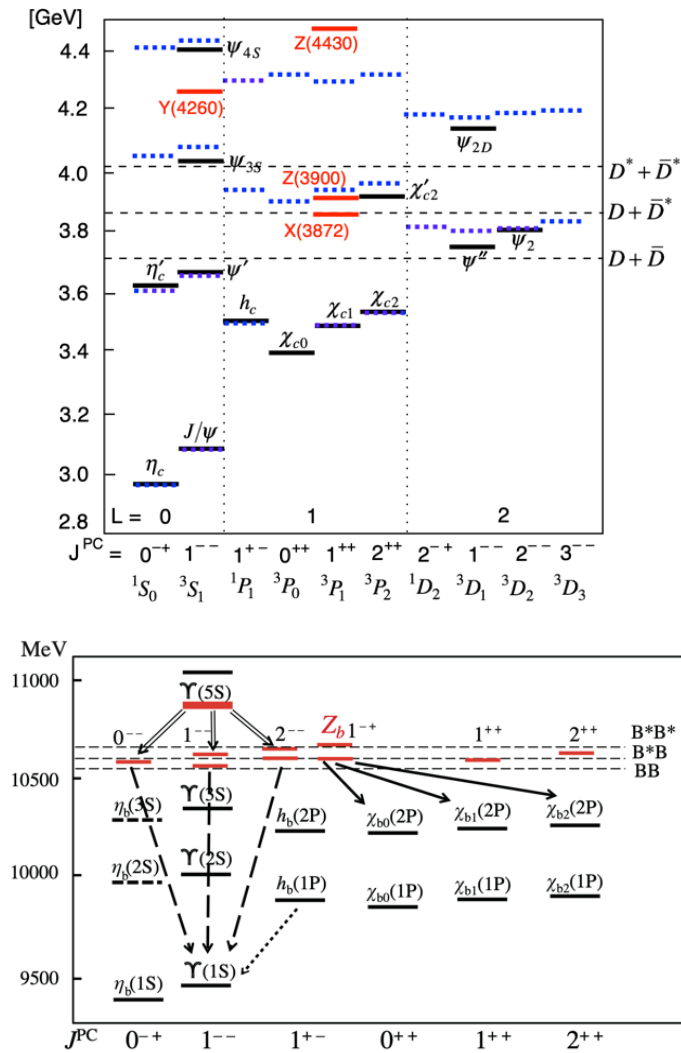
Fig. 28-1: Spectroscopies of charmonium (top) and bottomonium (bottom) 864 .
