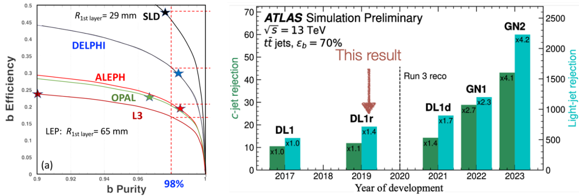
Fig. 15-12: Performances in heavy flavour tag at LEP (left) 410 and ATLAS at LHC (right) 411 .
