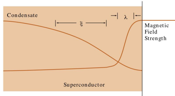
Fig. 7.6: The Higgs mechanism and superconductivity 186 .
