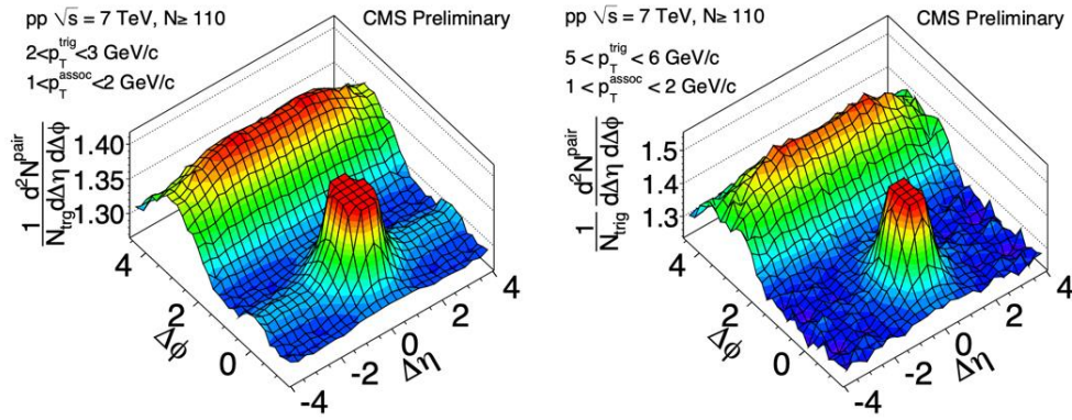
Fig. 20-14: Two-dimensional (2-D) per-trigger-particle associated yield of charged hadrons as a function of \Delta\eta and \Delta\phi with jet peak cut-off for better demonstration of the ridge from high multiplicity ( N \geq 110 ) pp collisions at \sqrt{s} = 7 TeV, for (a) 2 < p_T^{\text{trig}} < 3 GeV and 1 < p_T^{\text{assoc}} < 2 GeV and (b) 5 < p_T^{\text{trig}} < 6 GeV and 1 < p_T^{\text{assoc}} < 2 GeV.
