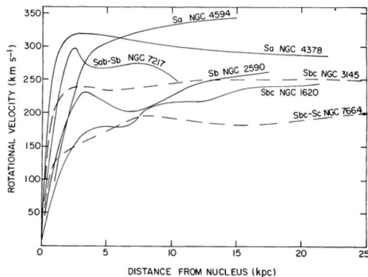
Fig. 31-1: Historical plot of Vera Rubin in 1978 991 .
