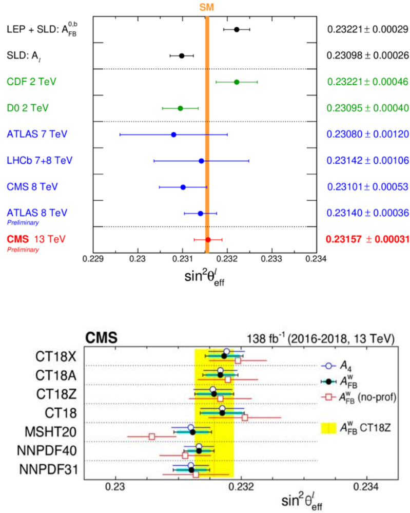
Fig. 24-33: Top: all measurements of the weak angle 771 . Bottom influence of PDF's choice on the result 772 .
