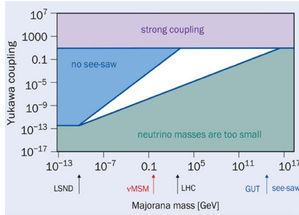
Fig. 19-17: Trading coupling against mass 539 .
