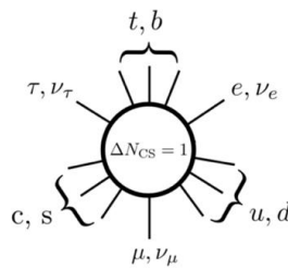
Fig. 24-21: The diagram of flavour of the process related to a unit change in Chern–Simons number, \Delta \mathbf{N}_{CS} = 1 .
