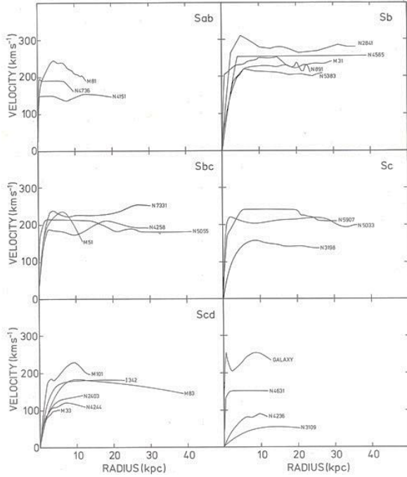
Fig. 31-2: Historical plots of rotational curves from different galaxies of A. Bosma 992 .
