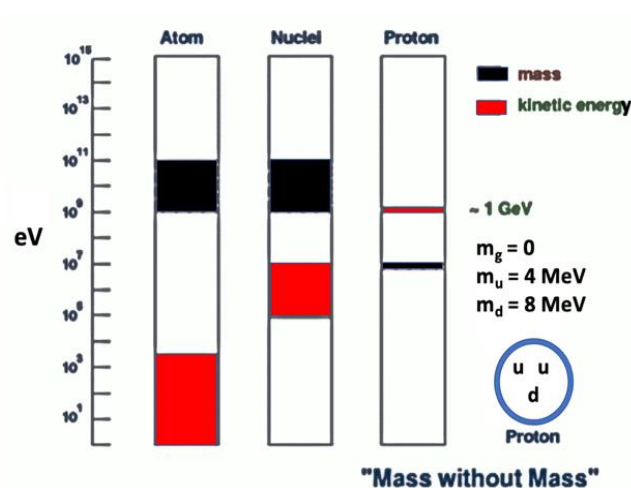
Fig. 7-8: Mass and kinetic energy from atom to proton.
