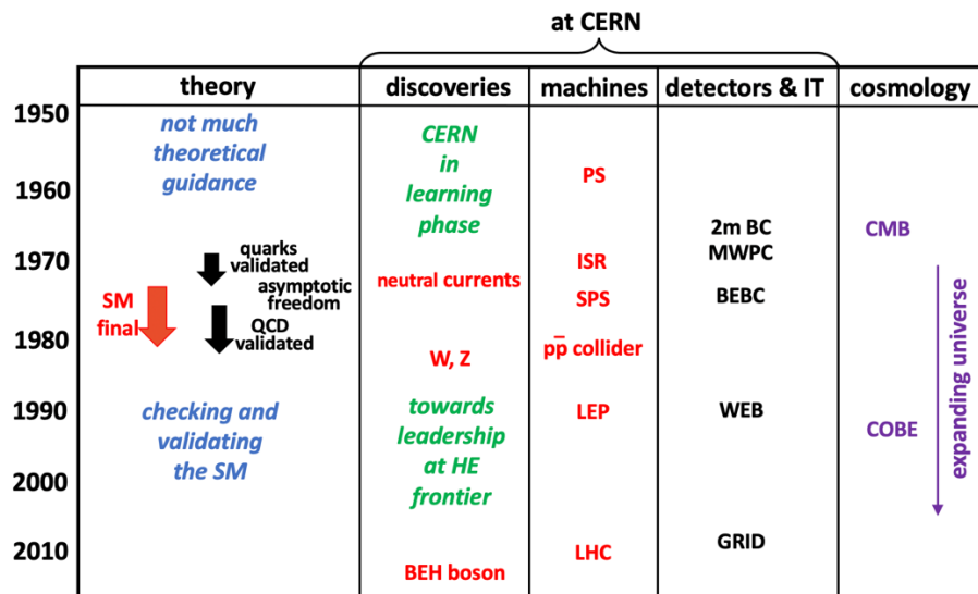
Fig. 2-1: Schematic outline of the adventure seen from CERN. For the broad view see Fig. 2-4. Figure by D. Treille.
