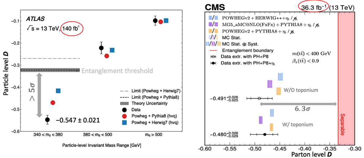
Fig. 24-43 Left: ATLAS evidence for entanglement 790 . Right: CMS measurement of the D parameter 791 .
