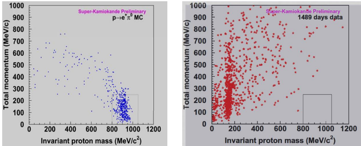
Fig. 32-29: The present limit on p \rightarrow e^+ \pi^0 is 2.4 \times 10^{34} years. Left is the signal MC and right are the data. The black box shows the signal region.
