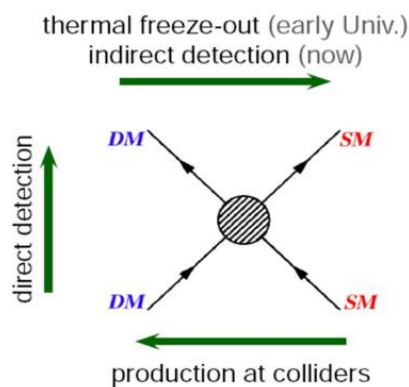
Fig. 31-11: The three types of DM searches 1015 .
