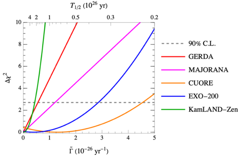
Fig. 32-5: \Delta\chi^2 profiles for experiments versus the 0\nu\beta\beta inverse half time (bottom abscissa) and half-life (top abscissa) of related isotope 1114 .
