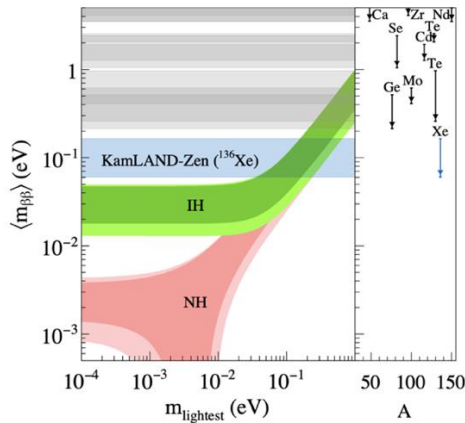
Fig. 32-3: The effective mass \langle m_{\beta\beta} \rangle versus the presently unknown lightest neutrino mass 1110 .
