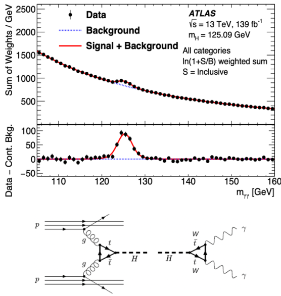
Fig. 24-1: The 2-photon mass spectrum 687 .
