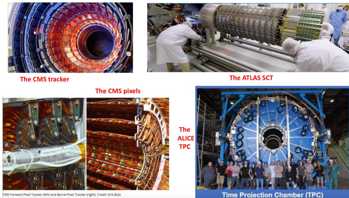
Fig. 23-12: The LHC trackers 673 .
