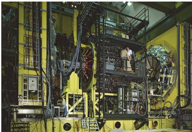
Fig. 12-3: UA2 detector (left) and its silicon pad detector (right).
