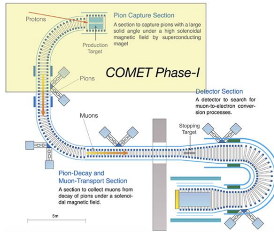
Fig. 32-25: COMET at J-PARK, Japan.
