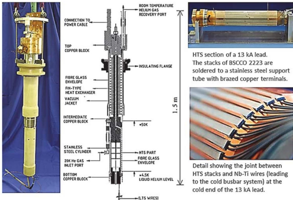
Fig. 23-6: Details on the warm superconducting current entries, a major achievement 667 .
