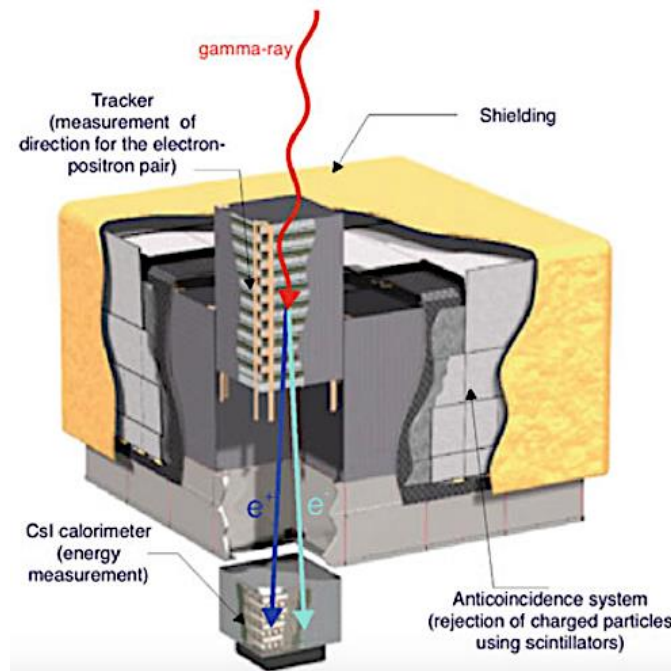
Fig. 35-9: Schematic diagram of the LAT.
