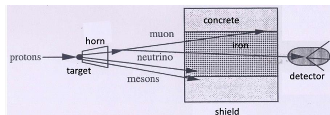
Fig. 9-1: The set-up.
