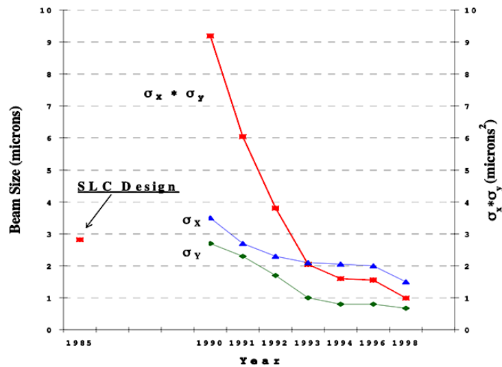
Fig. 15-4: Evolution of beam size at the SLC interaction point.
