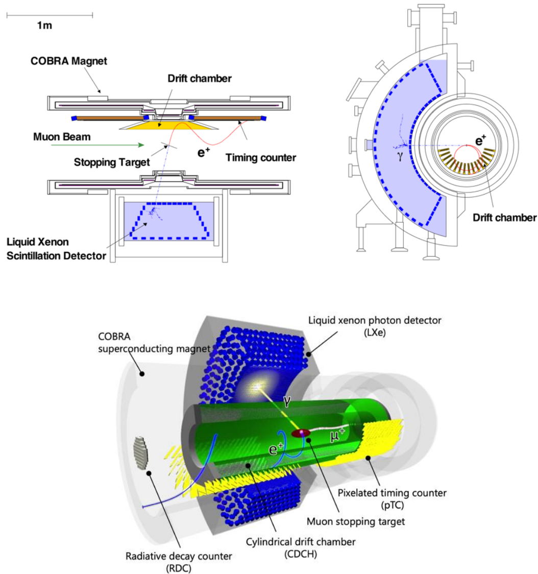
Fig. 32-23: The MEG (top) and MEGII (bottom) experiments.
