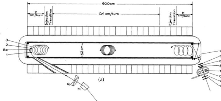
Fig. 26-10: The magnet of the first experiment.
