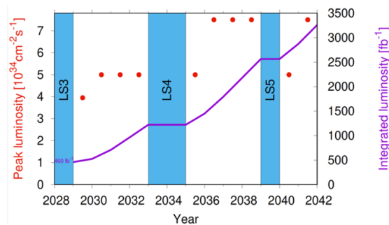
Fig. 22-6: Prospects for the peak and integrated luminosity for LHC 655 .
