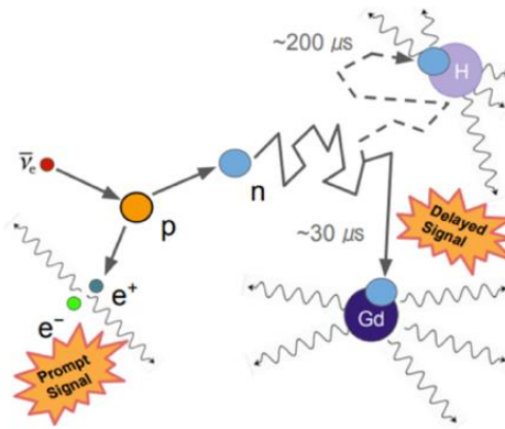
Fig. 19-34: Principle of reactor measurement 592 .
