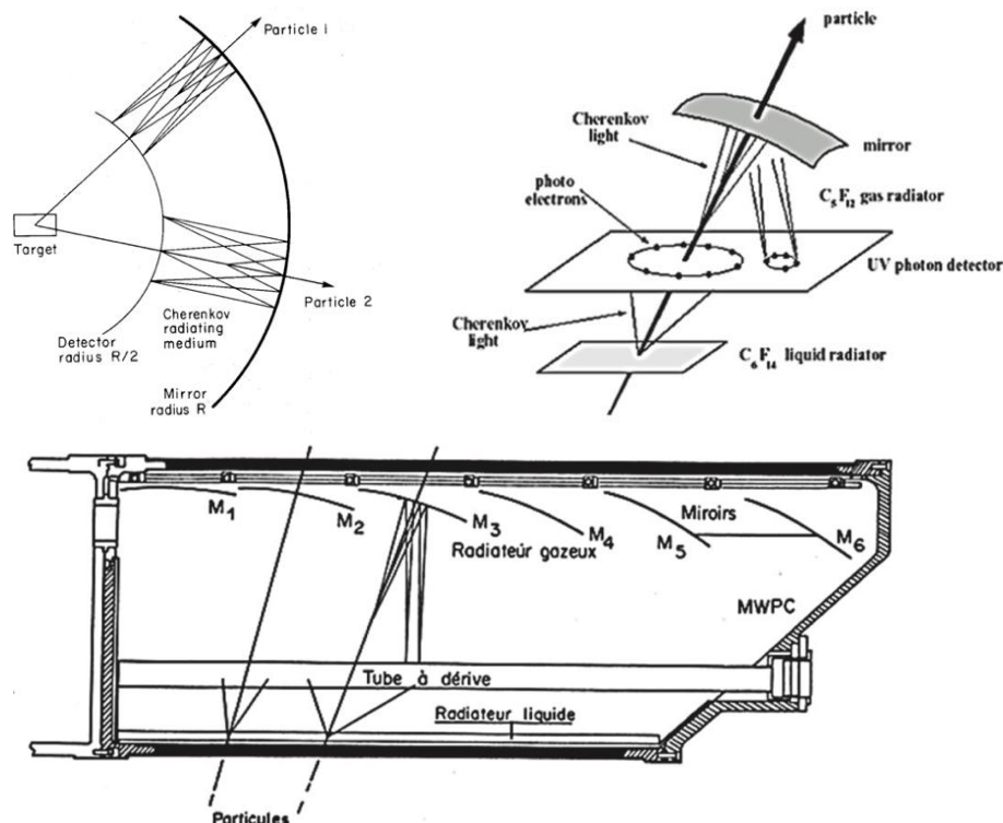
Fig. 6-2: The RICH 105 saga: Upper Left: the original idea of a spherical device. Upper right: the two-radiator arrangement. Bottom: sketch of the DELPHI Barrel Rich. Drift length of 155 cm.
