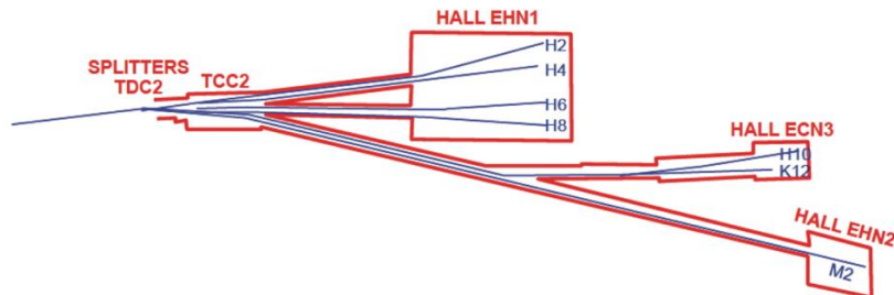
Fig. 10-5: The North Area beam lines.
