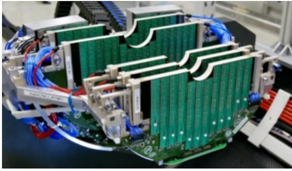
Fig. 23-2: ALICE muon spectrometer.
