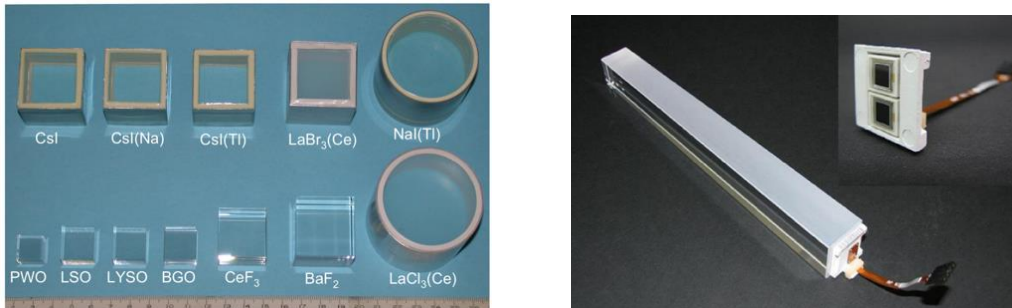
Fig. 6-7: Left: Picture showing twelve crystal scintillators with dimension of 1.5 X_0 124 . Right: Picture of a PbWO 4 crystal (about 28 X_0 with photodetector attached), used in CMS.
