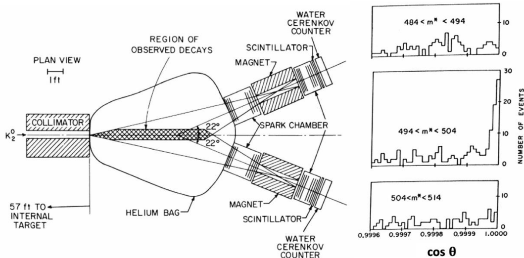
Fig. 13-2: Indirect CP violation: Nobel Prize in 1980 to James Cronin and Val Fitch. The set-up (left) and the signal (right).
