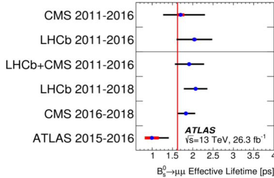
Fig. 8-7: B_s^0 \rightarrow \mu^+ \mu^- effective lifetime (ps) 206 .
