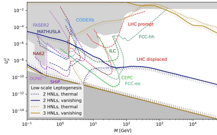
Fig. 19-25: Range consistent with both see-saw and leptogenesis 560 .
