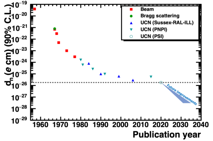
Fig. 32-15: Evolution of the nEDM results and projected future improvements 1129 .
