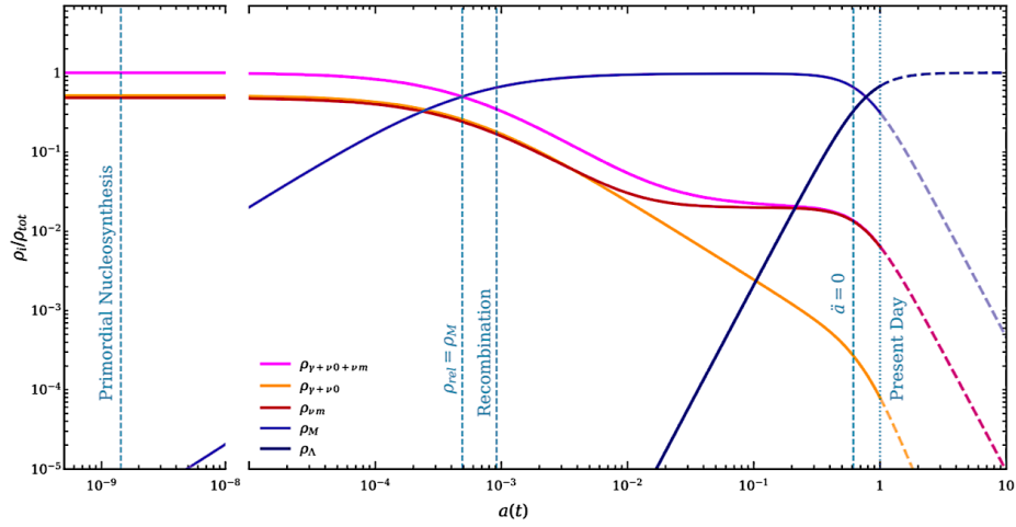
Fig. 19-38: The contributions to the total energy density of the Universe from different components as a function of the scale factor a(t) 596 .
