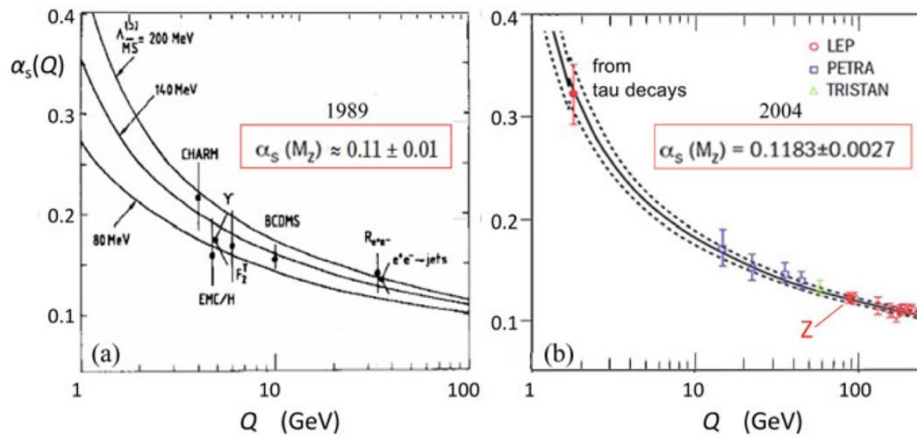
Fig. 16-5: The situation of the strong coupling before and after LEP 424 .
