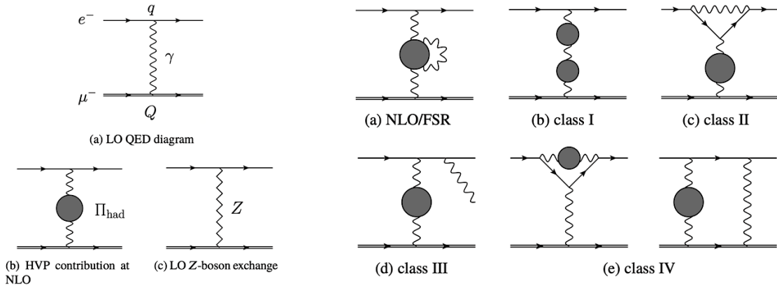
Fig. 26-21: Left: LO contributions; right: diagrams contributing at NLO (a) and NNLO (b-e) 852 .
