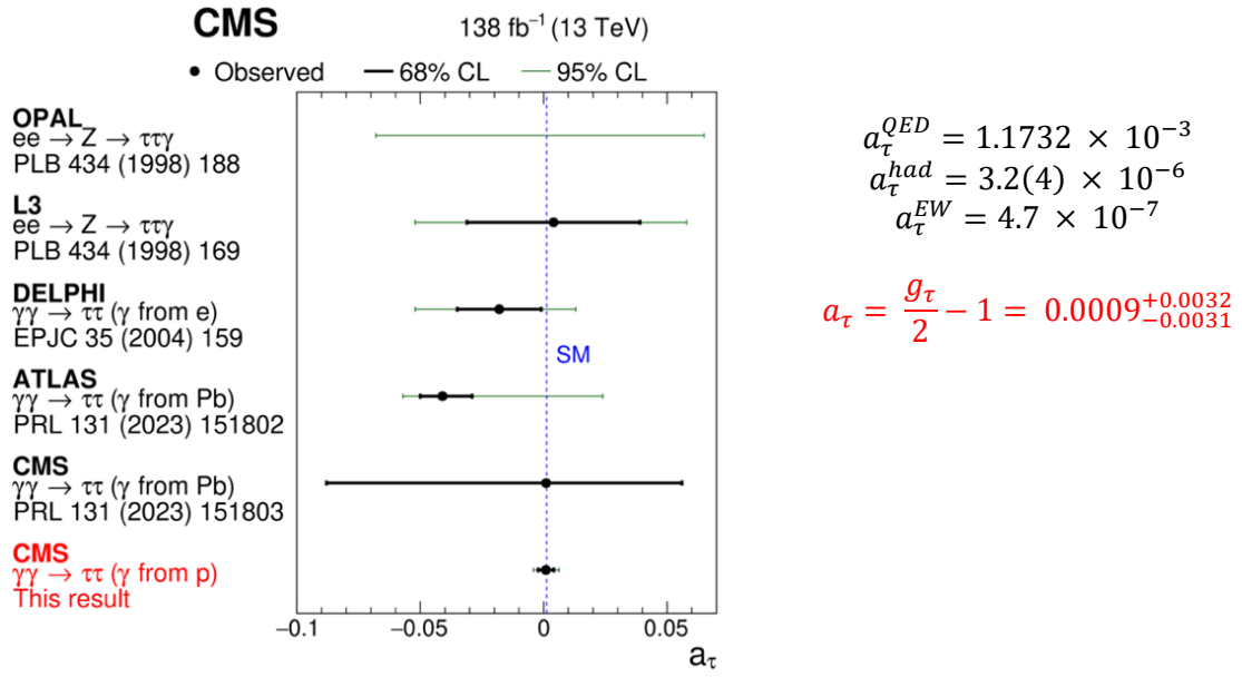
Fig. 26-15: g-2 of the tau (left), present measurement and expected components (right).
