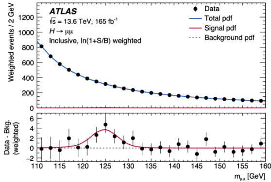
Fig. 24-9: Left: ATLAS results on H \rightarrow \mu\mu 701 ; right: CMS upper limit on H \rightarrow c\bar{c} 702 .
