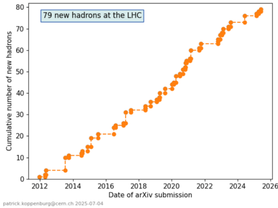
Fig. 22-7: An avalanche of new hadrons 656 .
