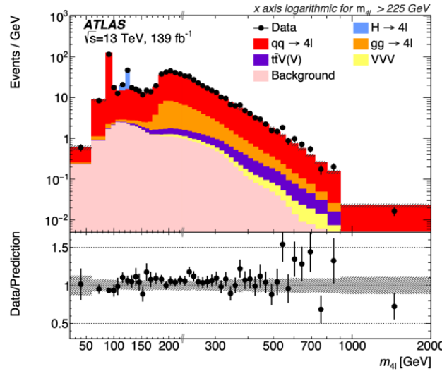
Fig. 24-23: The ATLAS 4-lepton spectrum, which stirred some turmoil 741 .
