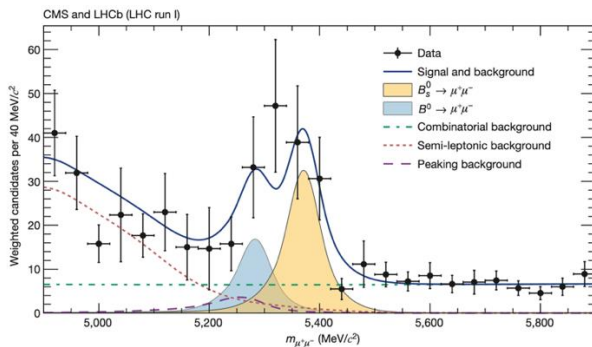
Fig. 8-4: Status of neutral B^0 \rightarrow \mu^+\mu^- decays 203 .
