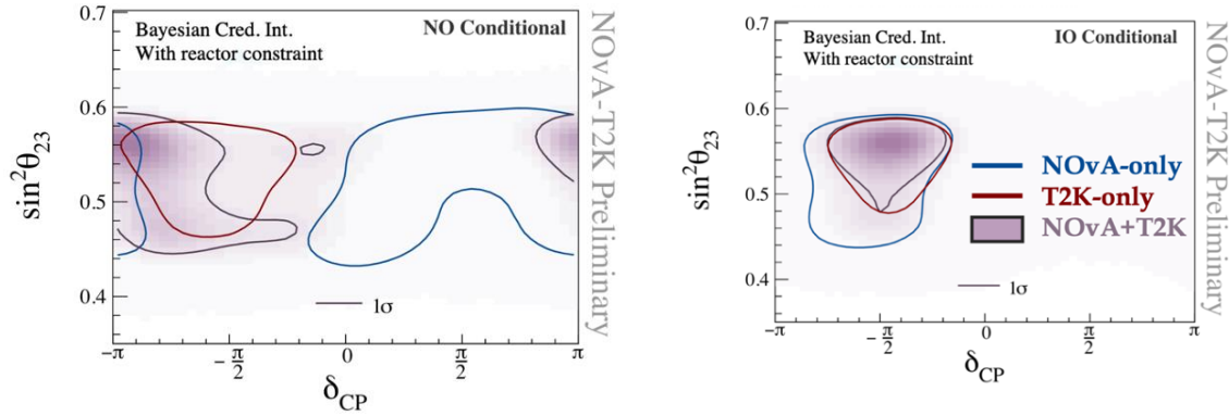
Fig. 19-15: NOvA and T2K results 529 : Left: mild preference for Inverted Ordering but influenced by \theta_{13} constraint. Right: CP-conserving points are outside 3\sigma intervals if ordering is inverted.
