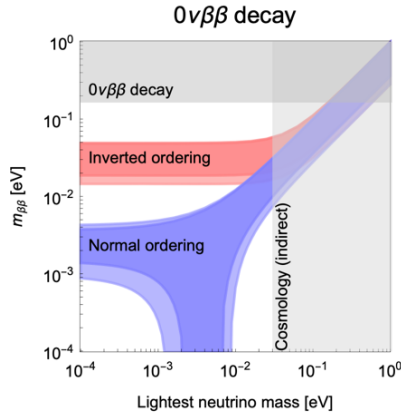
Fig. 19-8: m_{\beta\beta} versus lightest \nu mass from 0\nu\beta\beta .
