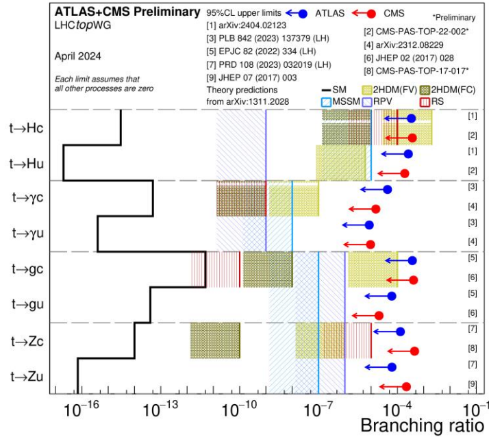
Fig. 8-9: Limits on top FCNCs 207 .
