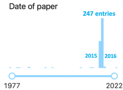
Fig. 24-26: The “750 GeV”, 247 entries in the INSPIRE data base in 2015 and 2016.
