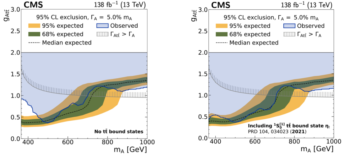
Fig. 24-45: Search for heavy scalar or pseudoscalar states in t\bar{t} events at CMS. The effect at top threshold (left) is no more visible when a model of toponium is introduced (right) 798 .
