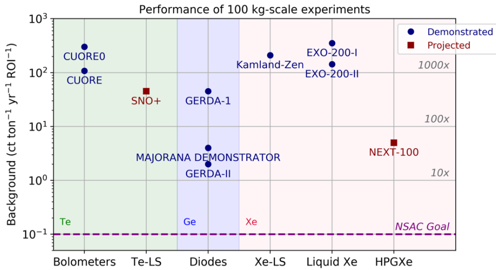
Fig. 32-6: Approximate background indices in present (100kg scale) programmes 1115 .
