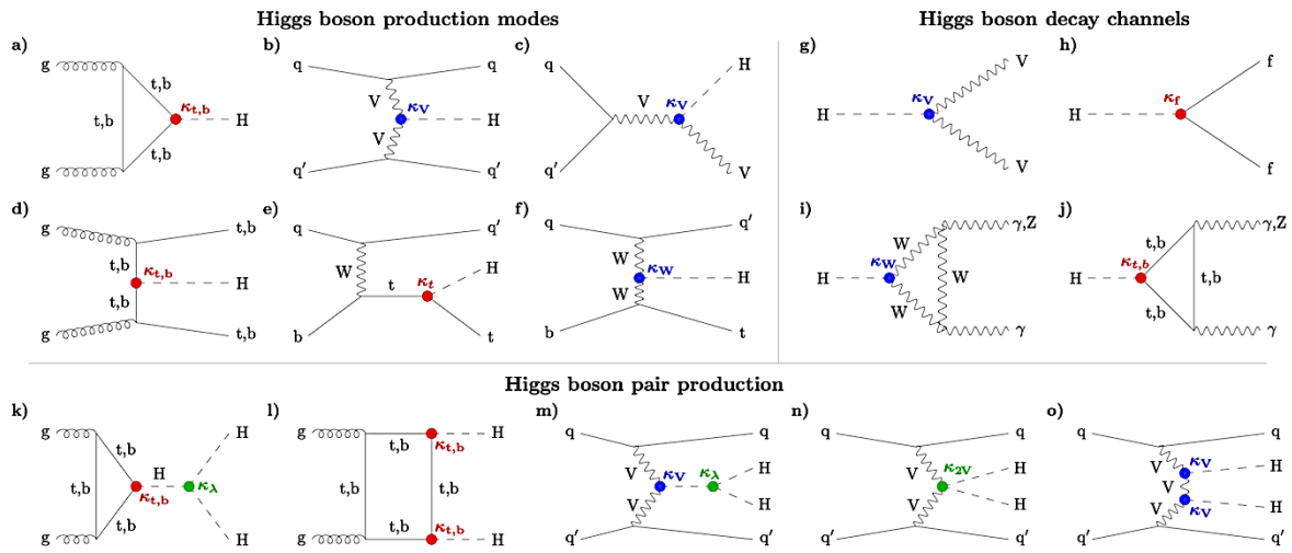
Fig. 24-6: The Feynman diagrams for the leading Higgs boson interactions. See text for explanations 693 .
