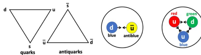
Fig. 4-4: The quark model.
