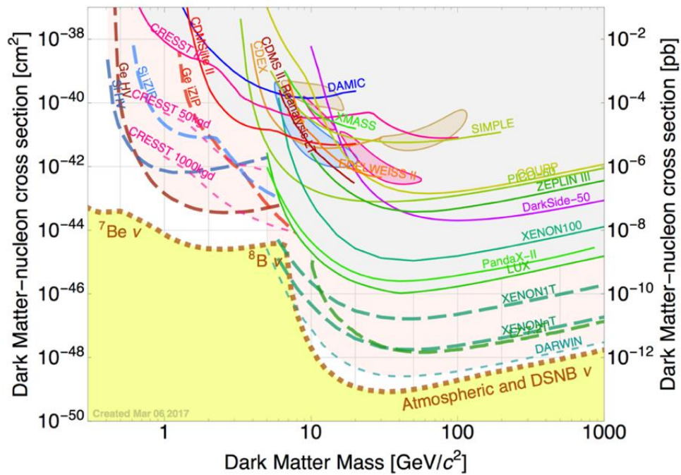
Fig. 31-19: DM-nucleon cross-section as function of the DM mass. Exclusion limits reached 1022 .
