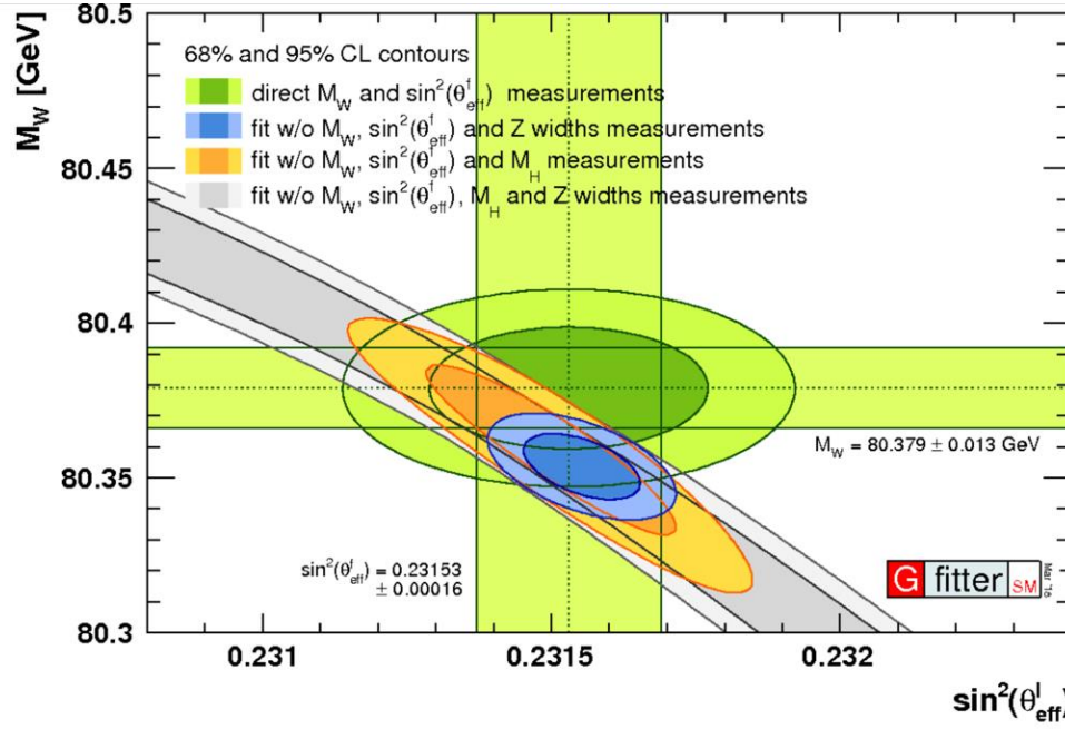
Fig. 24-51a: The confidence-level contours of the indirect determination of the W and \sin^2(\theta_{\text{eff}}^I) from the global EW fit compared to the measurements of M_W and \sin^2(\theta_{\text{eff}}^I) .
