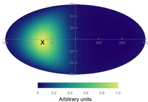
Fig. 31-26: Map of the WIMP flux in Galactic coordinates. The direction of v_{lab} is indicated as a cross on the map.
