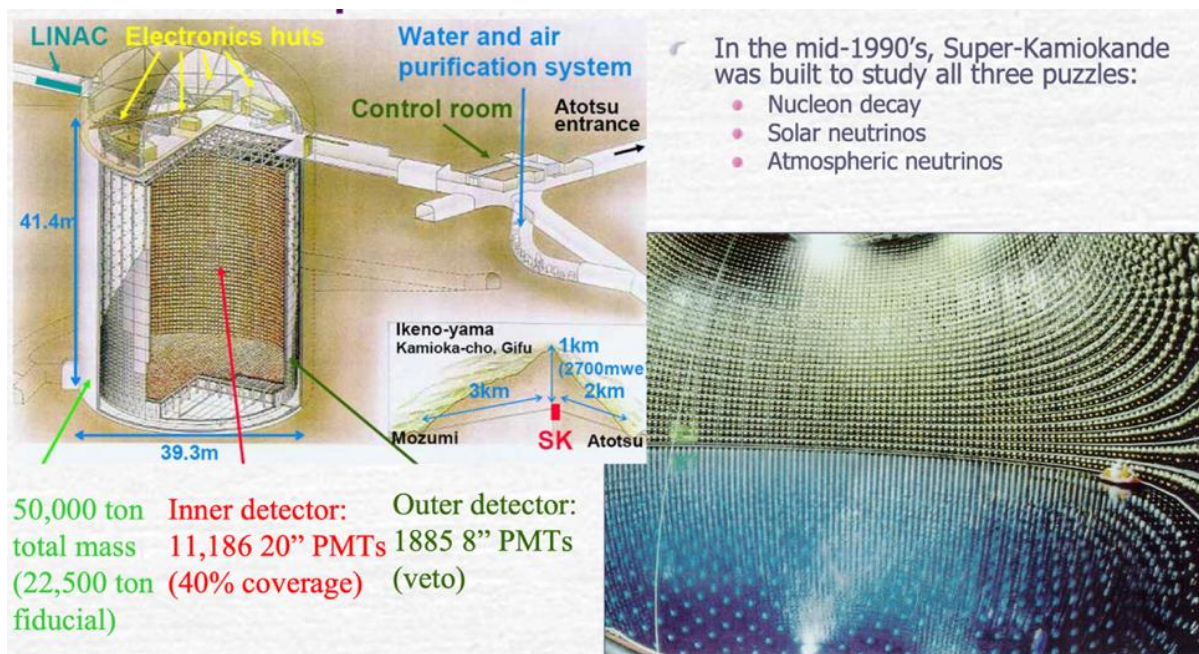
Fig. 32-28: The Super-Kamiokande detector 1161 .
