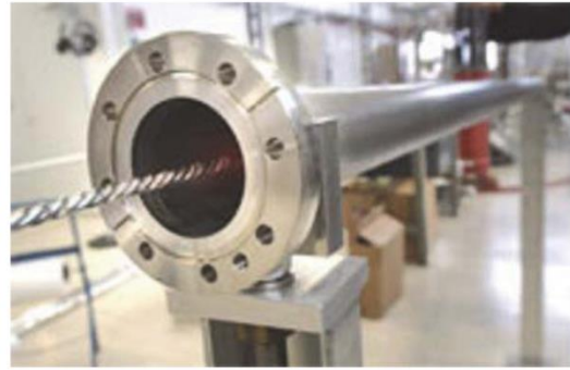
Fig. 23-5: Beam screen and vacuum tube coating 666 .
