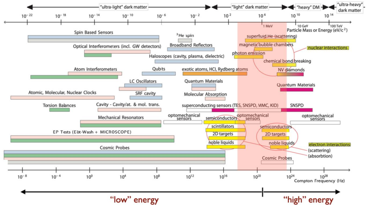
Fig. 31-42: Ranges of applicability of different quantum sensor techniques to search for BSM physics 1070 .
