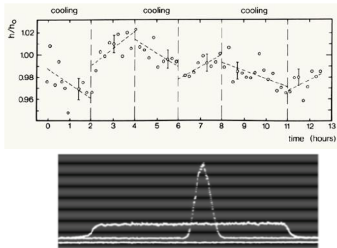
Fig. 10-9: Top: cooling at ISR; bottom: in momentum at ICE.
