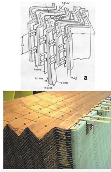
Fig. 23-10: The ATLAS accordion: its structure and the organisation of its construction 671 .
