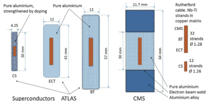
Fig. 6-8: Structure of the superconductors of the ATLAS and CMS solenoids at LHC 127 .
