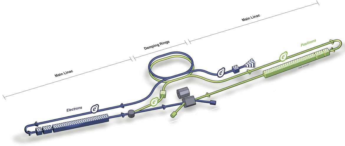
Fig. 3.3: Conceptual layout of the LCF/ILC collider.
