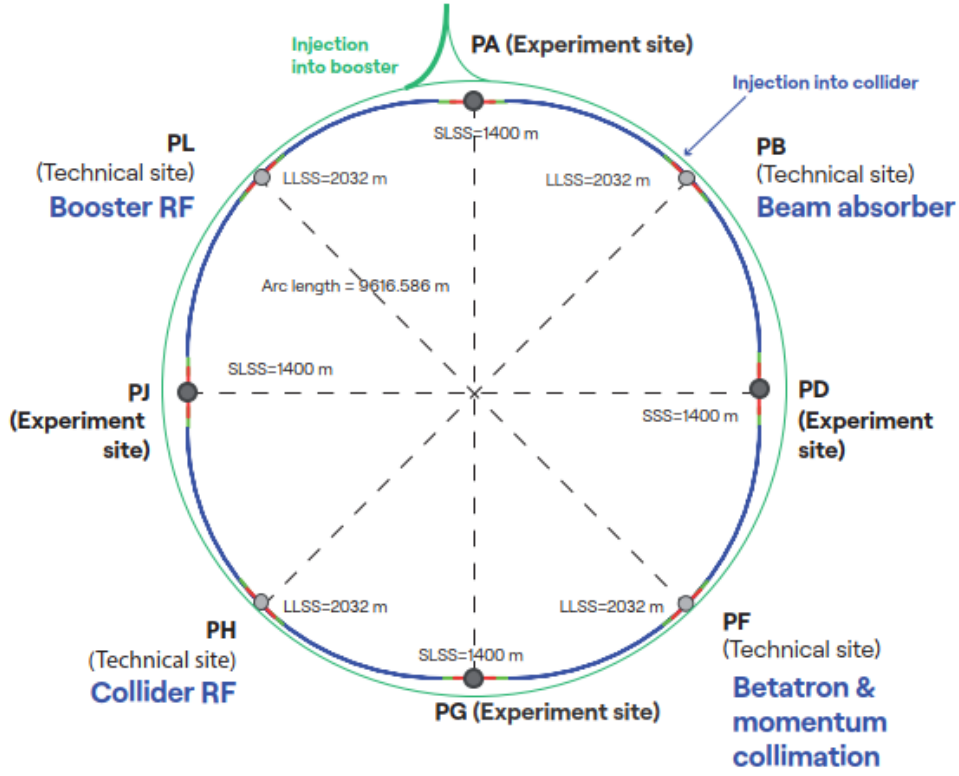
Fig. 3.2: Schematic diagram of the FCC-ee collider.
