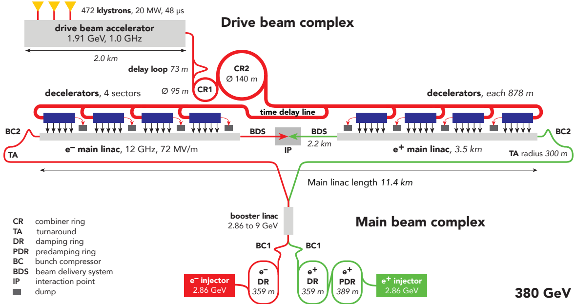
Fig. 3.1: Conceptual layout of the CLIC collider (380 GeV).
