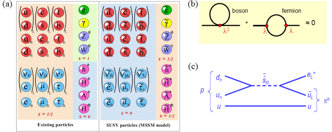
Fig. 80: (a) The increased particle content of supersymmetry, where the super-partners of the SM particles (known as sparticles) are indicated with a \sim over their symbol; (b) the cancellation of divergent terms; (c) a diagram that would allow proton decay.
