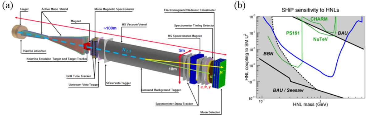
Fig. 99: (a) The proposed SHiP spectrometer, with a decay of an HNL illustrated; (b) sensitivity of SHiP to HNLs in the plane of coupling vs mass [143].
