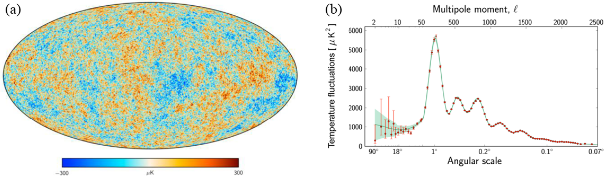
Fig. 5: (a) Fine structure seen in the temperature fluctuations of the cosmic microwave background; (b) analysis of the corresponding observed power spectrum, compared to the model [10].
