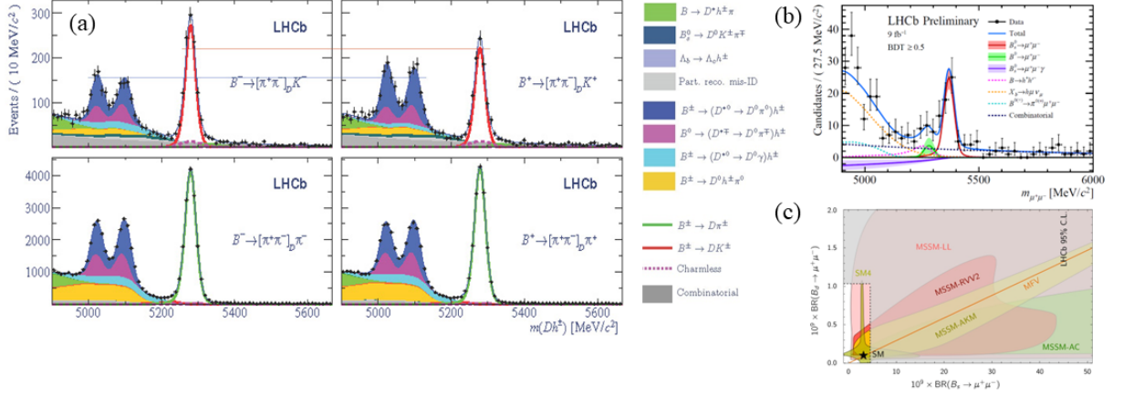
Fig. 65: (a) Analysis of B \rightarrow Dh decays showing clear CP violation [85]; (b) signal for the very rare decay B_s^0 \rightarrow \mu^+\mu^- [86]; (c) constraints on the parameter space for new physics models, as a result of the measurements of B^0 and B_s^0 \rightarrow \mu^+\mu^- [87].
