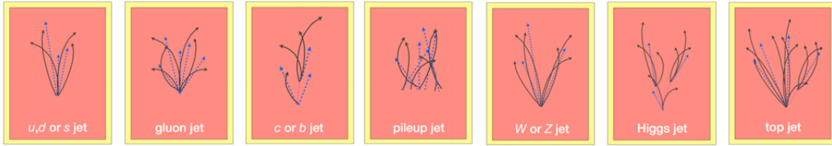
Fig. 51: Sketches of jet topologies corresponding to different underlying processes [22].
