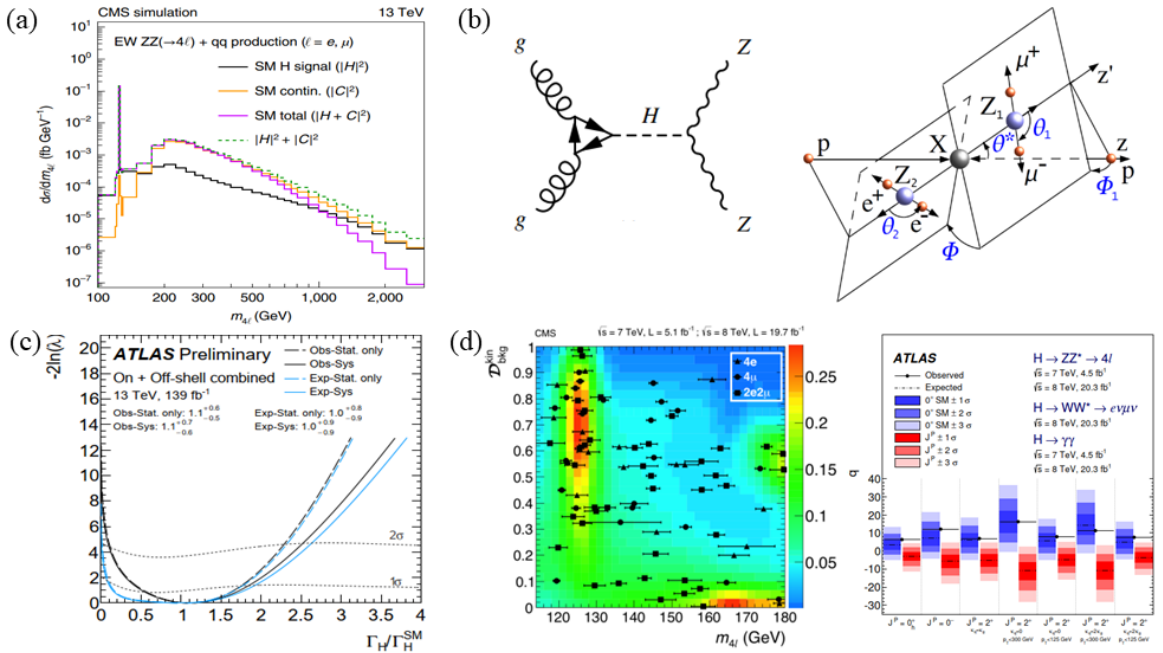
Fig. 73: (a) Simulated mass distribution for H \rightarrow ZZ^* \rightarrow 4\ell , showing the on-shell (peak at 125 GeV) and off-shell production [100]; (b) the gluon-fusion production diagram for H \rightarrow ZZ (left) and definition of decay angles for analysis of ZZ \rightarrow 4\ell (right); (c) measured likelihood as a function of \Gamma_H/\Gamma_H^{\text{SM}} [101]; (d) observed data are compared to discriminant distributions to calculate a likelihood for different spin states (left) and different hypotheses are tested (right, where the SM is blue and alternative spin hypotheses red) [103].
