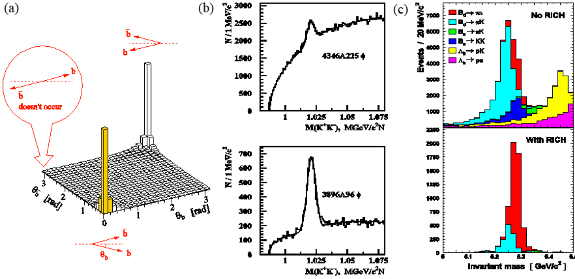
Fig. 39: (a) Correlation between production angle of b and \bar{b} quarks at the LHC: the acceptance of LHCb is shaded yellow; (b) improvement in signal to background ratio when using a RICH detector to select \phi \rightarrow K^+K^- decays [45]; (c) importance of particle identification in separating two-body B decays, such as B^0 \rightarrow \pi^+\pi^- (shaded red), without use of RICH (above) and with RICH (below) [46].
