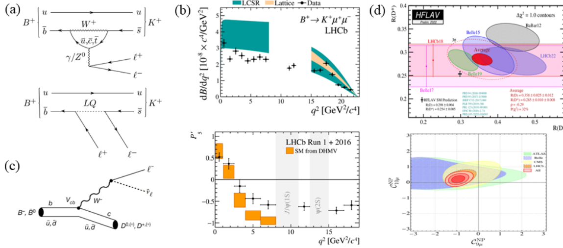
Fig. 89: (a) Diagrams for b \rightarrow s \ell^+ \ell^- decays in the SM (above) or for a model involving leptoquarks (below); (b) discrepancies seen in such decays vs the momentum transfer q^2 for the rate [124] (above) and one of the many angular distributions [125] (below); (c) tree diagram for B^0 \rightarrow D^{(*)} + \ell \nu ; (d) combination of results on R_{D^*} vs R_D [126] (above) and of all anomalies vs coefficients for new physics [127] (below).
