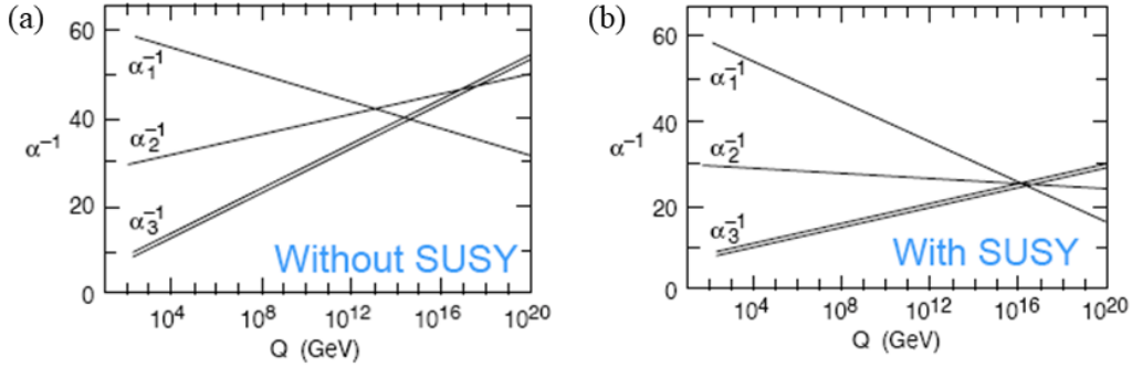
Fig. 81: Extrapolating the coupling “constants” to high energy scale (a) in the SM; (b) adding supersymmetry [113].
