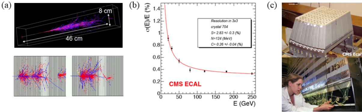
Fig. 29: (a) Simulation of an electromagnetic shower (above) and hadronic shower (below), where the less uniform energy deposition of the latter can be seen, the EM component shown in red comes from \pi^0 \rightarrow \gamma\gamma decays; (b) energy resolution of the CMS ECAL; (c) crystals of the CMS ECAL (above) and construction of the ATLAS Tilecal (below) [34].
