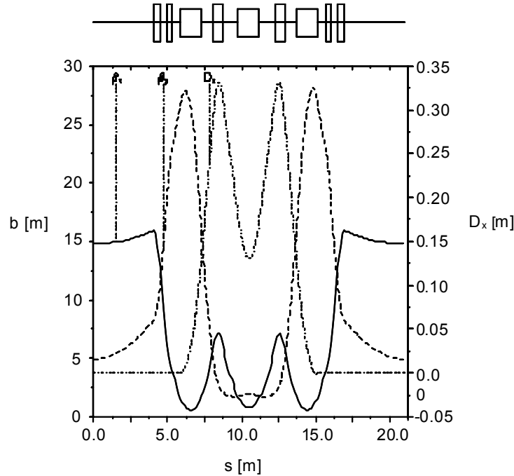
Figure 3.2.11: Betatron functions in horizontal and vertical planes, with the dispersion function along one cell.
